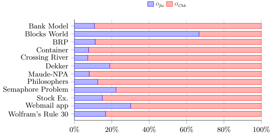
Figure 5: Overhead comparison O_{fix} vs. O_{Chk} .
