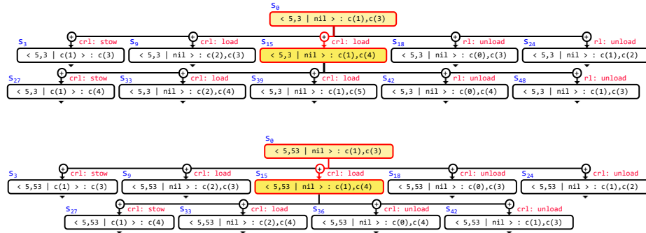
Figure 4: (Above) Fragment of the computation tree of the CONTAINER-TERMINAL module. (Below) Fragment of the computation tree of the CONTAINER-TERMINAL-FIX module.
