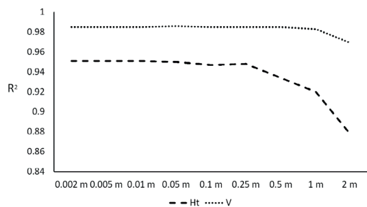
Figure 3. Determination coefficient variation for total height ( Ht ) and crown volume ( V ) estimation for subsampled distances from 0.002 m to 2 m.
