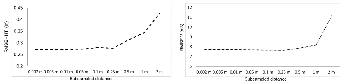
Figure 4. Variation of RMSE for total height ( Ht ) and crown volume ( V ) estimation for subsampled distances from 0.002 m to 2 m.
