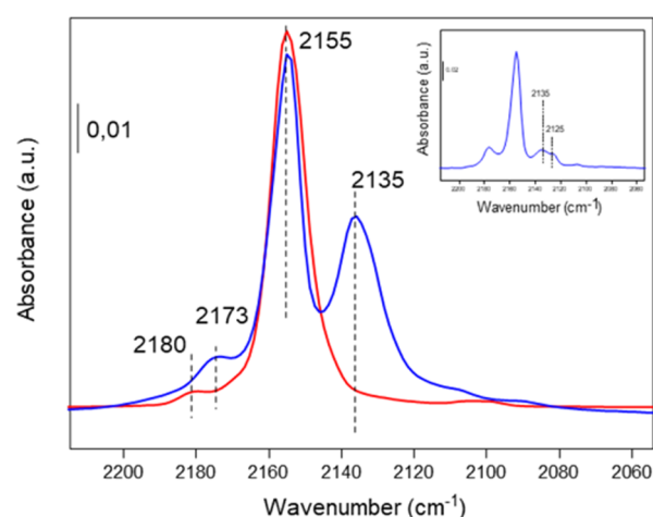
Figure 2. IR spectra of CO adsorption at -165 °C at saturation coverage (2 mbar) on nanoceria (red) and UiO-66 (Ce) (blue). The inset IR spectrum of CO adsorption at 0.5 mbar on the UiO-66 (Ce) sample.
