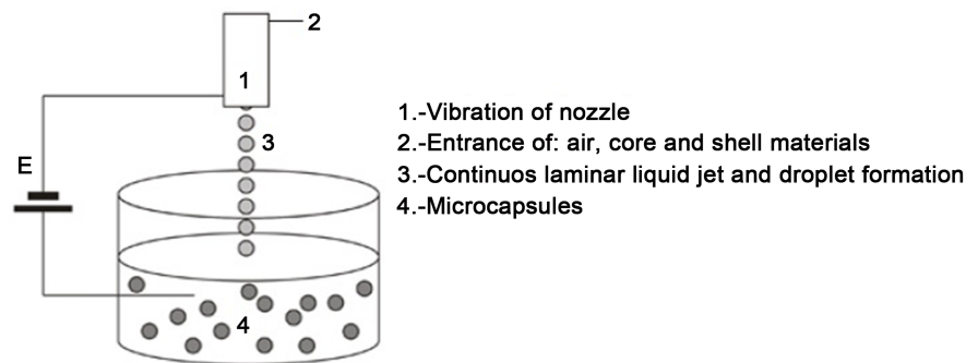
Figure 1. Microcapsules formation.
