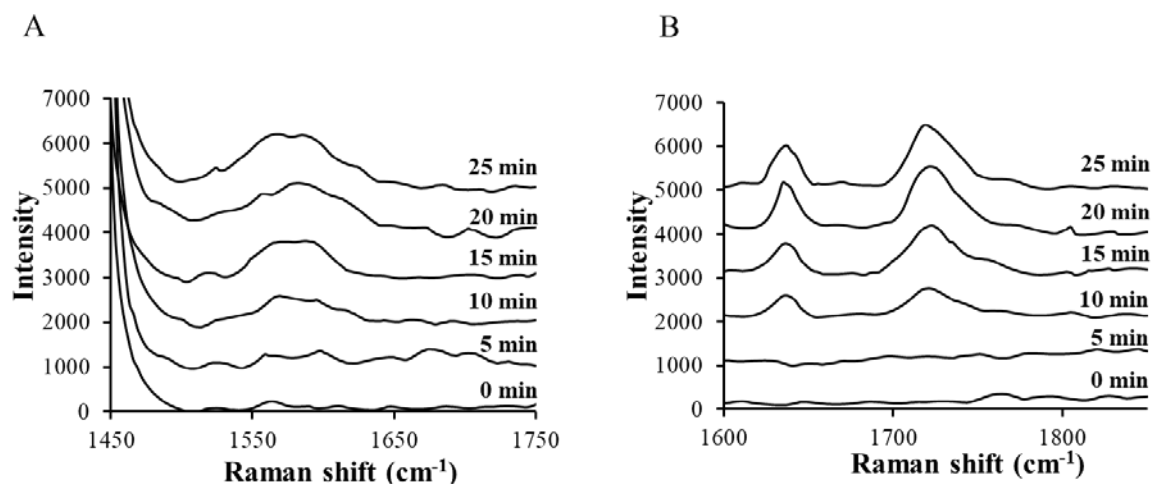
Fig. 3. Raman spectra of the inner ETFE tubing treated with: (A) BP and (B) EDMA at several UV irradiation times. The grafting EDMA experiments were conducted using each time as starting material a 20 min BP-treated ETFE material.
