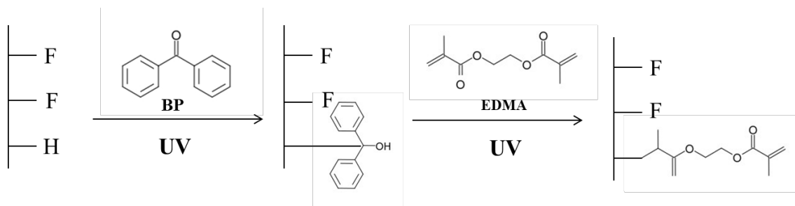
Fig. 2. Two-step photografting scheme for chemical modification of ETFE tubing.
