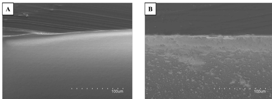
Fig. 4. Photographs and SEM micrographs of ETFE tubing untreated (A) and grafted with EDMA layer (B).
