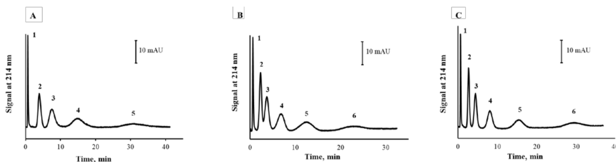
Fig. 6. Separation of alkyl benzenes on several polymer monoliths in an ETFE tubing: (A) poly(STY-co-DVB), (B) poly(BMA-co-EDMA) and (C) poly(GMA-co-DVB). Experimental conditions: 100 mm \times 0.75 mm i.d.; mobile phase, 33%(v/v) ACN in water; flow rate, 0.3 mL min -1 ; injection volume, 1 \mu L; UV at 214 nm. Peak identification: (1) uracil, (2) toluene, (3) ethylbenzene, (4) propylbenzene, (5) butylbenzene, (6) pentylbenzene.
