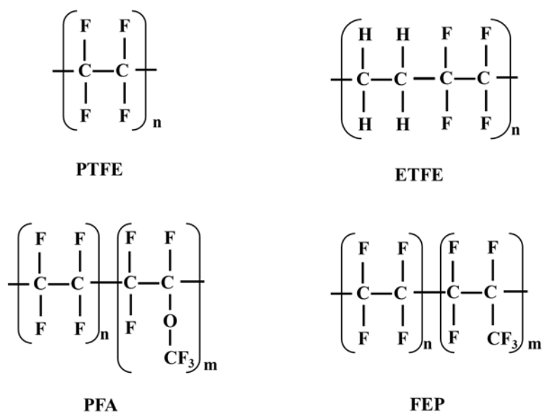
Fig. 1. Structures of fluoropolymers investigated in this study.
