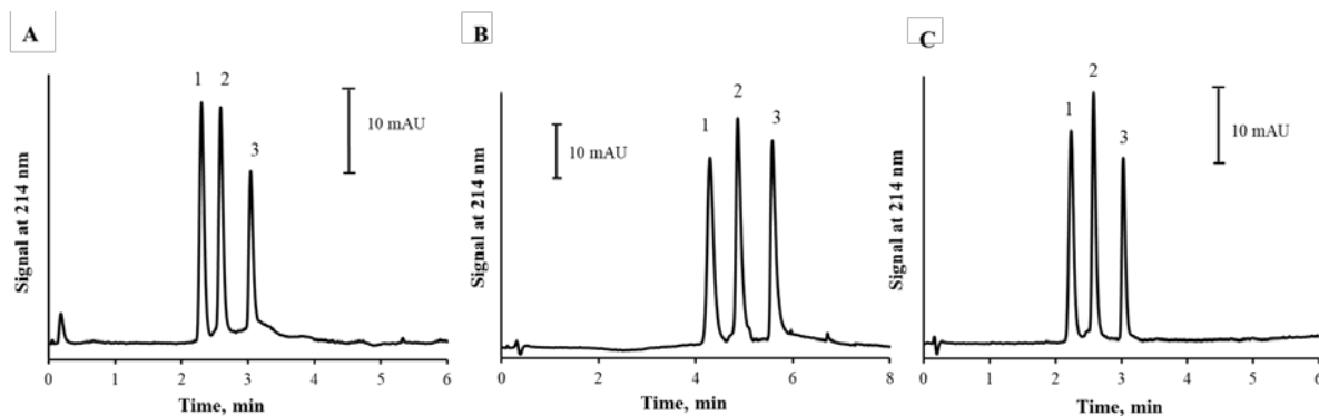
Fig. 7. Separation of proteins on several polymer monoliths in an ETFE tubing: (A) poly(STY-co-DVB), (B) poly(BMA-co-EDMA) and (C) poly(GMA-co-DVB). Experimental conditions: mobile phase, A = 0.1% aqueous TFA, B = 0.1% TFA in ACN; linear gradient from 17 to 100% B in A in 5 min at 1 mL min -1 (trace A); linear gradient from 17 to 60% B in A in 5 min at 0.5 mL min -1 (trace B); linear gradient from 17 to 100% B in A in 5 min at 1 mL min -1 (trace C); other experimental conditions as in Fig. 6. Peak identification: (1) ribonuclease A, (2) cytochrome C and (3) myoglobin.
