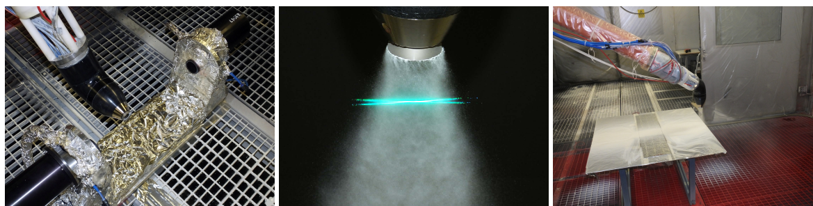
(a) Measurement of particle size distribution (b) 2-dimensional Laser-Doppler-Velocimetry (c) Spray pattern and transfer efficiency
