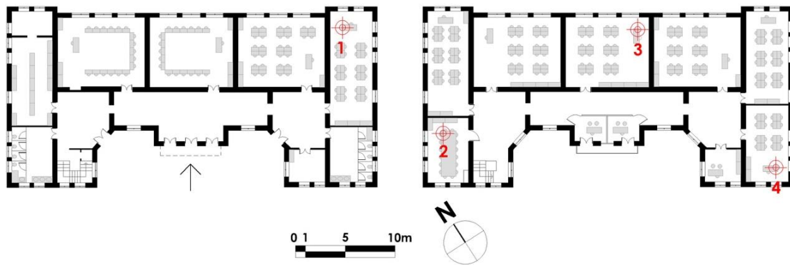
Figure 2 Building plans and dataloggers locations (ground floor on the left and first floor on the right). Note for Editor: two-column fitting image
