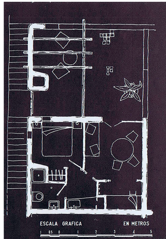
Figure 6. Top Left: Floor plan and elevation of Type A apartment. Original project (1956). Bottom Left: Floor plan and elevation of Type B apartment. Original Project (1956). Right: Floor plan of Type C apartment. Original Project (1956).
