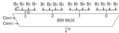
Fig. 6. Write circuit for the BW mechanism.
