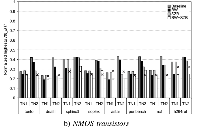
Fig. 20. Normalized highest dV_{th} caused by the BTI effect on the entire cache for each type of transistor. The cross symbol refers to the normalized highest dV_{th\_BTI} in the control bits.
