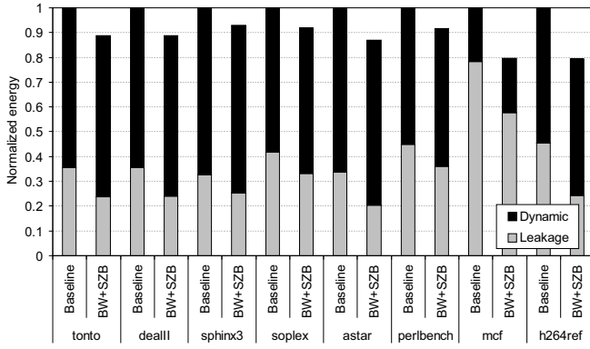
Fig. 18. Normalized consumption for the baseline and BW+SZB mechanisms.
