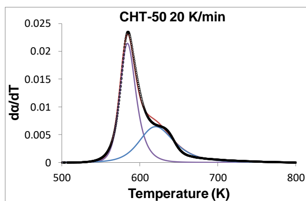
Figure 6. Experimental and fitted data of the derivative of the conversional degree for CHT-50 at 20 K/min, considering two peaks (□ Experimental, - - Sestak-Berggren fitting curve, - Peak 1 and - Peak 2). The fitted curve is superimposed to the experimental data. The contribution of each peak is also shown.
