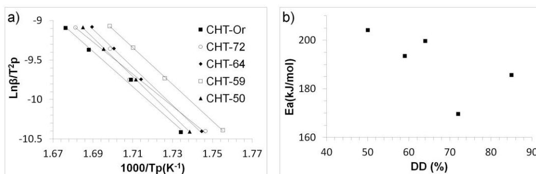
Figure 2. Kissinger plot of \ln\beta/T_p versus 1000/T_p for the chitosan and its N-acetylated derivatives (a); E_a values obtained from the slope of the straight lines (b).
