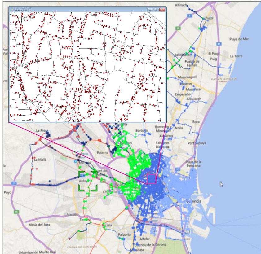
Figure 3. Building the Valencia's detailed model of 325,000 nodes, including house connections, by query. Red dots stand for demands in house connections.
