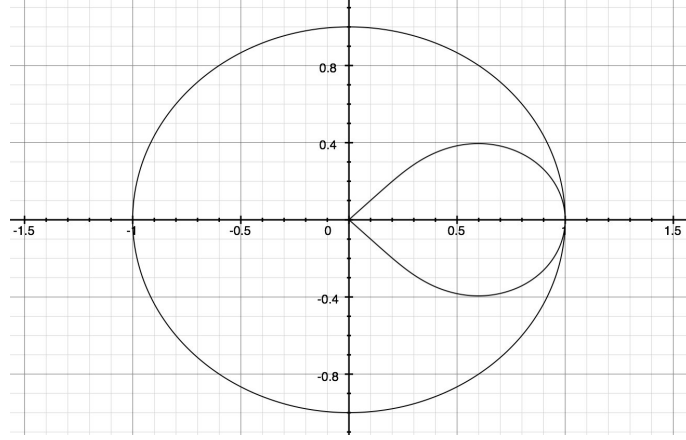
FIGURE 1. \delta(\mathbb{D}) for the symbol of the fractional second order backward difference scheme with \alpha = \frac{1}{2} and \tau = 4 , and \mathbb{T} .
