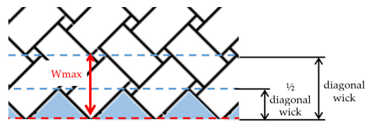
Figure 8. Theoretical maximum value of Wb in 45° fiber orientation tests.
