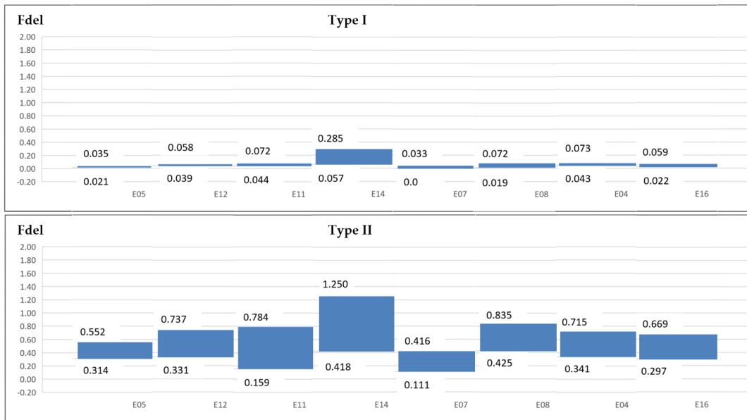
Figure 11. Fdel delamination factor.
