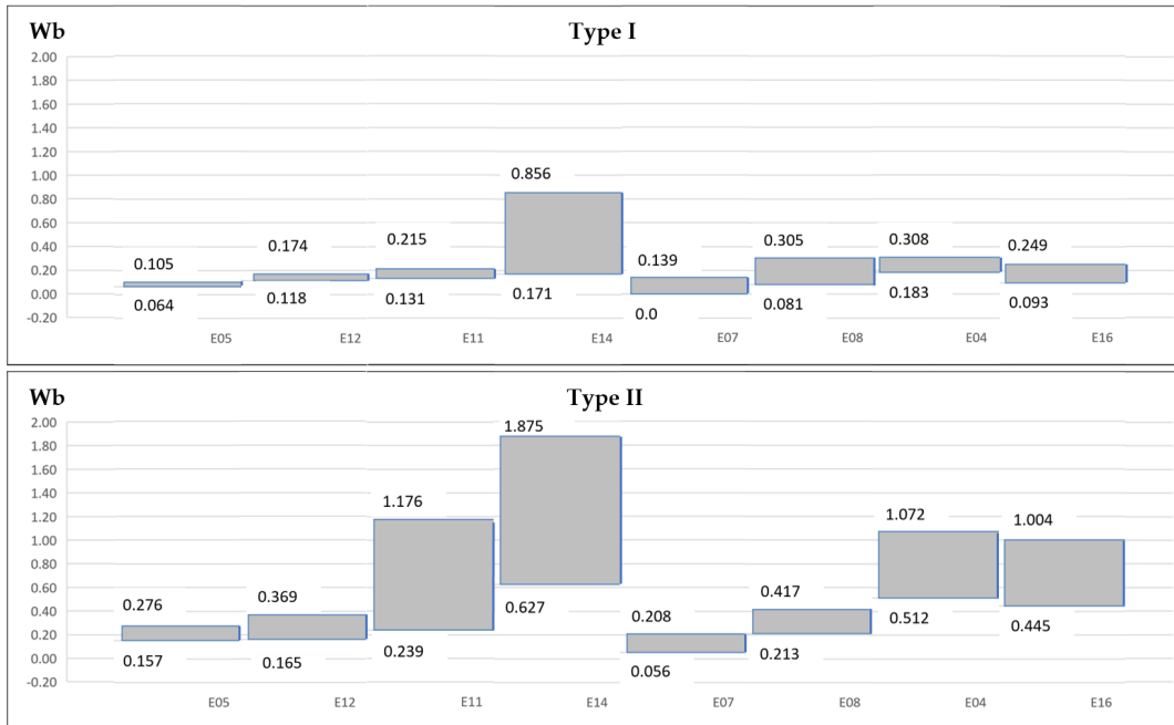
Figure 10. Wa and Wb delamination parameters.
