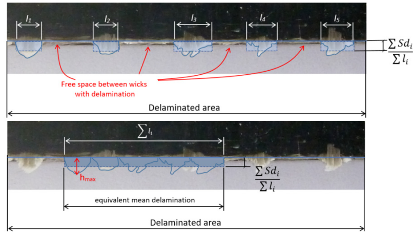
Figure 7. Equivalent delamination parameter (Wb) for Type II delamination.
