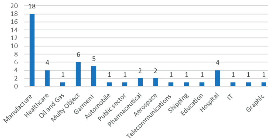
Figure 5. Research Object.
