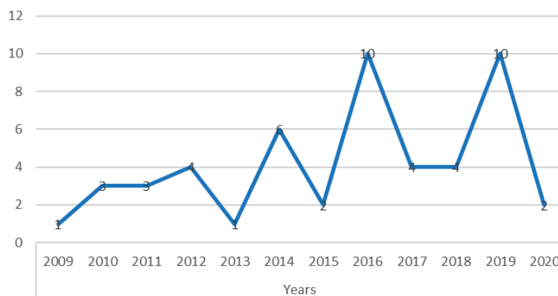
Figure 3. Years Publication.
