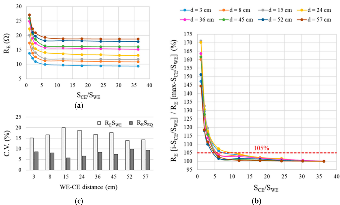
Figure 6. Electrical resistance ( R_E ) at different WE-CE distances in a saturated \text{Ca}(\text{OH})_2 solution with 0 \text{ mol}\cdot\text{L}^{-1} chlorides: (a) R_E vs. the S_{CE}/S_{WE} ratio; (b) R_E [i-S_{CE}/S_{WE}] / R_E [max-S_{CE}/S_{WE}] vs. S_{CE}/S_{WE} where R_E [i-S_{CE}/S_{WE}] is the R_E measured at the respective i-S_{CE}/S_{WE} and R_E [max-S_{CE}/S_{WE}] is the R_E obtained for the maximum S_{CE}/S_{WE} ; and (c) coefficient of variation in R_E \cdot S depending on whether S is defined as S_{WE} or S_{EQ} .
