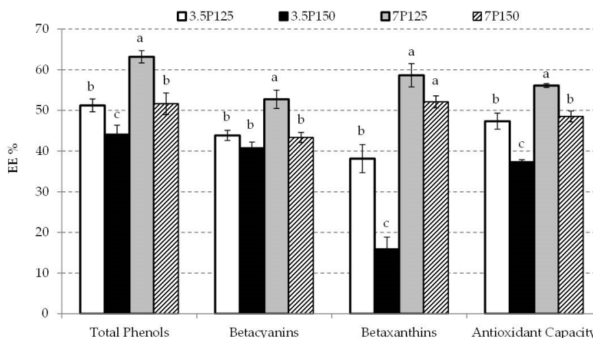
Figure 4. Mean values and standard deviation of encapsulation efficiencies percentage in beetroot spray-dried samples for analyzed bioactive compounds. Letters indicate homogeneous groups established by the ANOVA ( p < 0.05 ) for each bioactive compound or antioxidant capacity: 3.5P125 or 3.5P150, powder with 3.5% of pea protein concentration spray dried at 125 or 150 °C, respectively;
