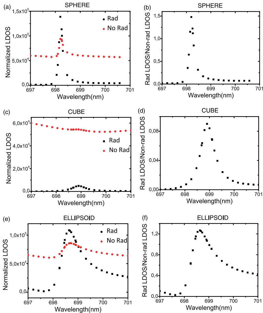
Fig. 18. Radiative and nonradiative contributions to the normalized LDOS for the (a) nanosphere-based ( R = 40 nm), (c) nanocube-based ( l = 75 nm), and (e) nanoellipsoid-based hybrid cavities ( w_c = 40 nm and l_c = 70 nm). In (b), (d), and (f) the ratio radiative/nonradiative LDOS is represented for the same configurations as in (a), (c), and (e).
