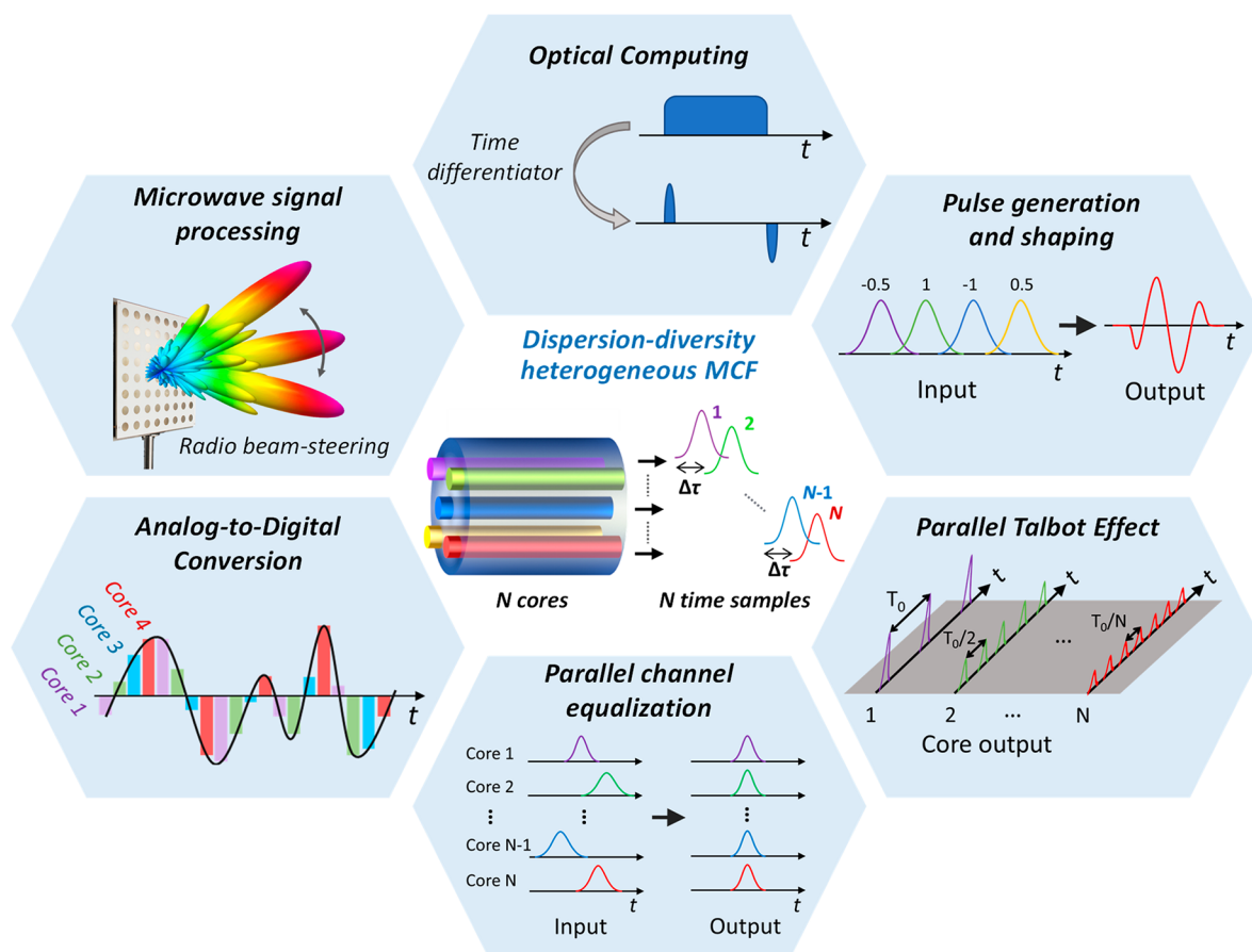
Figure 1. Representative examples of dispersion-diversity multicore fiber signal processing. The implementation of dispersion-diversity heterogeneous multicore fibers opens the door to a myriad of signal processing application fields.
