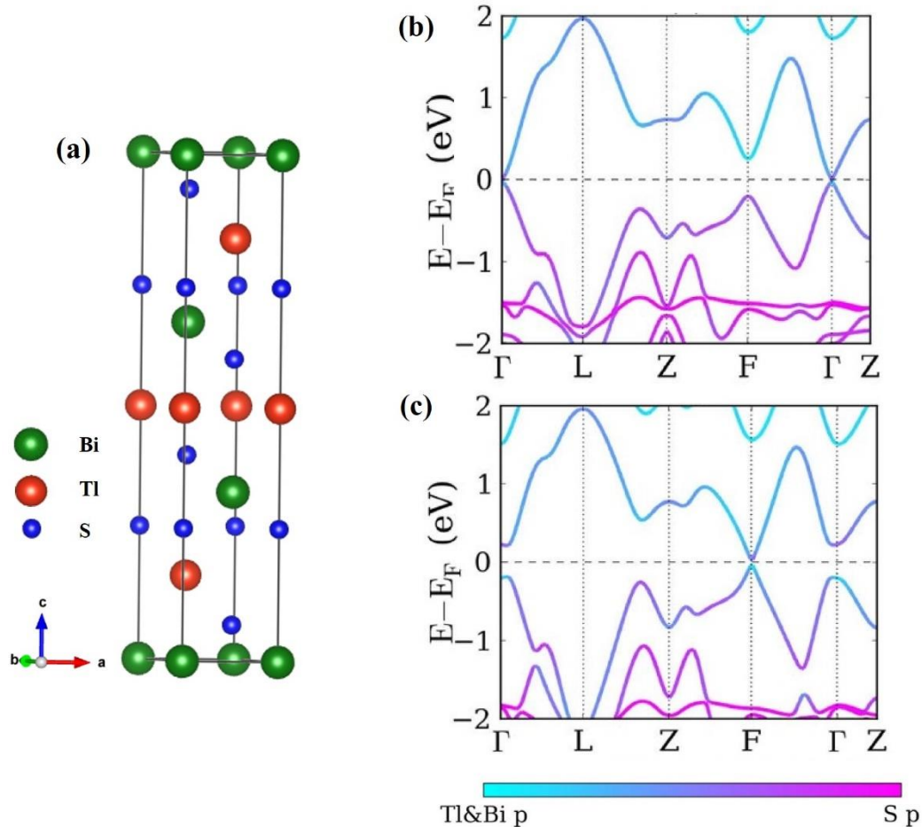
44 Figure 5. (a) Crystal structure of the rhombohedral phase of the \text{TlBiS}_2 compound. (b) The 45 calculated electronic band structure (including the SOC effects) of the \text{TlBiS}_2 at 0 GPa and 46 (c) 5.0 GPa. The first BI occurs at the \Gamma point of the BZ leading to the TI phase. The second 47 BI occurs at the F point of the BZ leading to the TCI phase. The color code represents the 48 contribution of orbital characters of Tl, Bi, and S atoms. This figure is adopted from Ref. 49 [20]. 50
