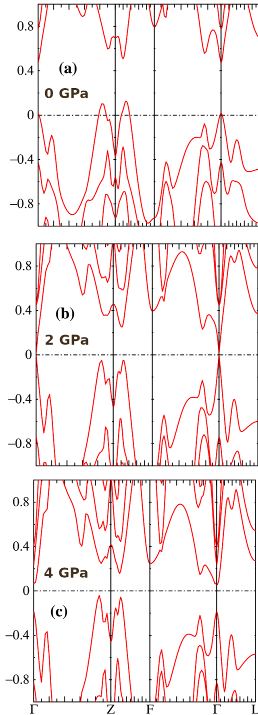
Figure 2. Theoretically calculated hydrostatic pressure dependent electronic band structure of \beta -As 2 Te 3 at (a) 0 GPa (top), (b) 2.0 GPa (middle), and (c) 4.0 GPa (down). The BI signature (W shaped) is evidenced at the \Gamma point of the BZ near to Fermi level. This figure is adopted from Ref. [7].
