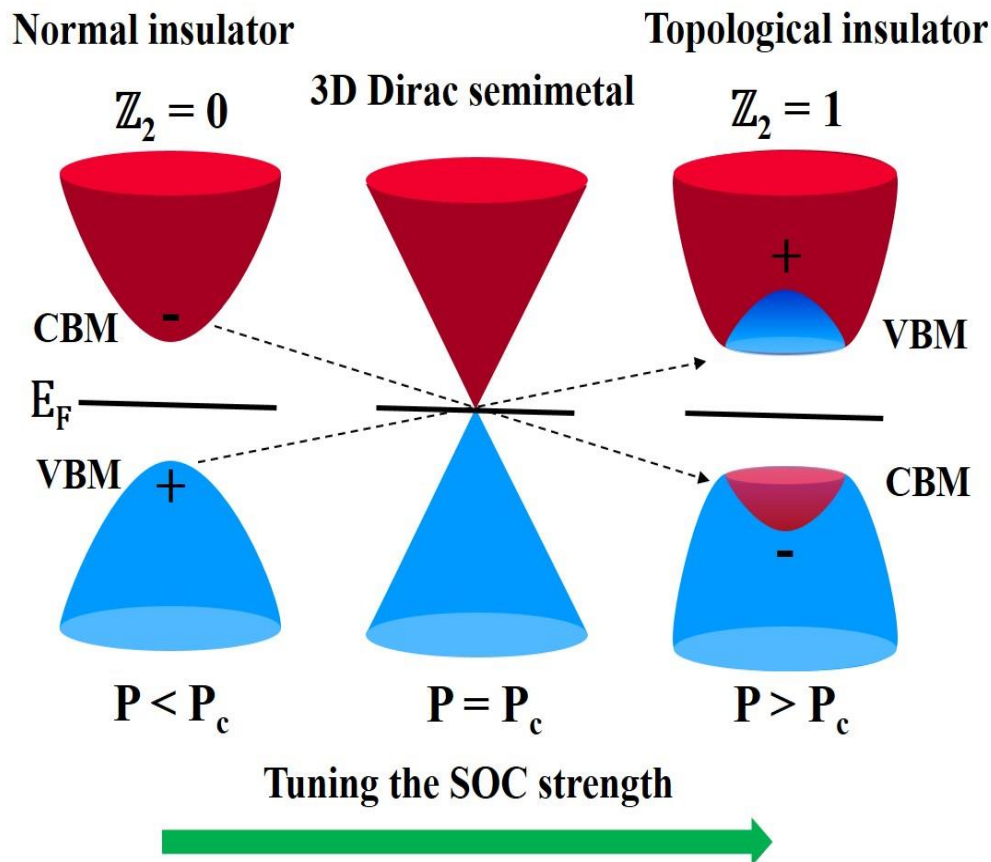
Figure 1. Schematic of the typical band inversion (BI) associated with the pressure-induced TQPT. The pressure-induced TQPT occurs due to the decrease, closing, and subsequent reopening of the band gap that occurs as pressure increases. This process usually occurs on increasing the SOC strength (for instance by chemical doping or substitution). Here, P_c represents the critical transition pressure at which the TQPT occurs because of the closing of the band gap. The - and + signs indicate the odd and even parity of the bands at the TRIM point, respectively. The BI is evidenced by the change in the parity of the valence band maximum (VBM) and conduction band minimum (CBM) that occurs above P_c .
