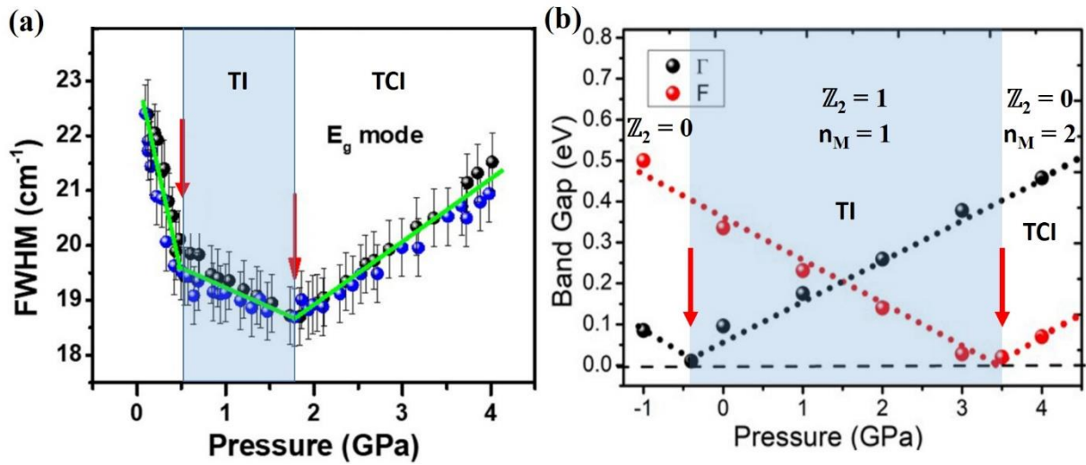
Figure 6. (a) Pressure dependence of FWHM of E_g mode in the rhombohedral phase of \text{TlBiS}_2 . The solid red arrow at \sim 0.5 GPa and \sim 1.8 GPa signature the TI and TCI phases, respectively. (b) Pressure vs. band gap at the \Gamma and F points of the BZ. The solid red arrow at \sim -0.4 GPa and \sim 3.6 GPa indicates the BI at \Gamma and F points of the BZ, respectively. The blue shaded region represents the TI phase. This figure is adopted from Ref. [40].
