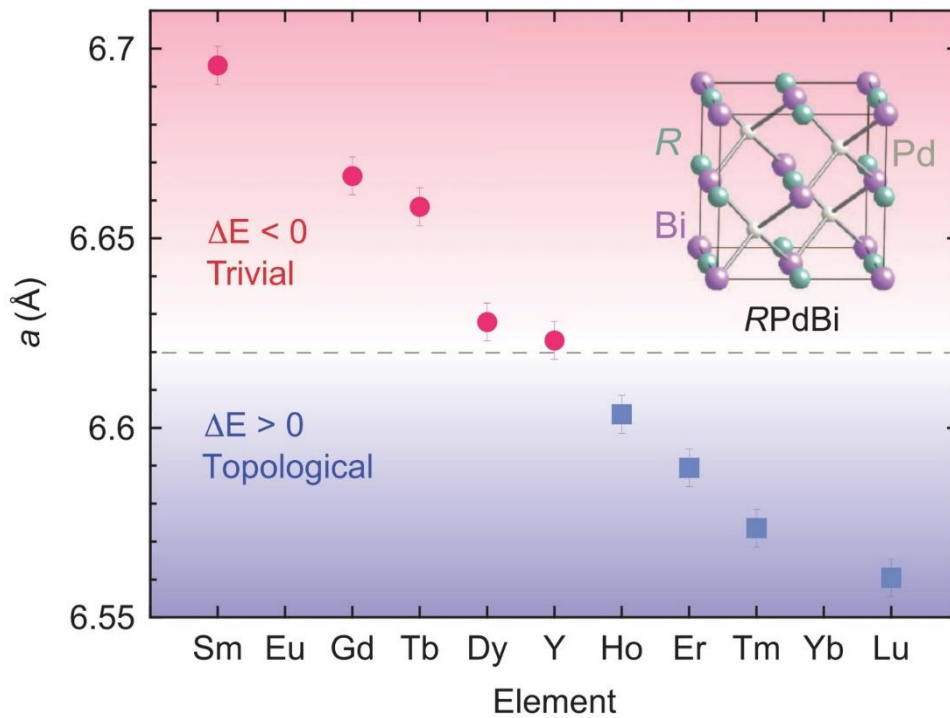
Figure 11. The plot of lattice parameter vs. lanthanides in half Heusler RPdBi compounds. Here, the dashed lines represent the critical value of the lattice parameter a_c = 6.62 \text{ \AA} . Below a_c ( \Delta E > 0 ), materials are TIs whereas above a_c ( \Delta E < 0 ), materials are NIs. The inset shows the cubic crystal structure of typical RPdBi compounds. This figure is adopted from Ref. [81].
