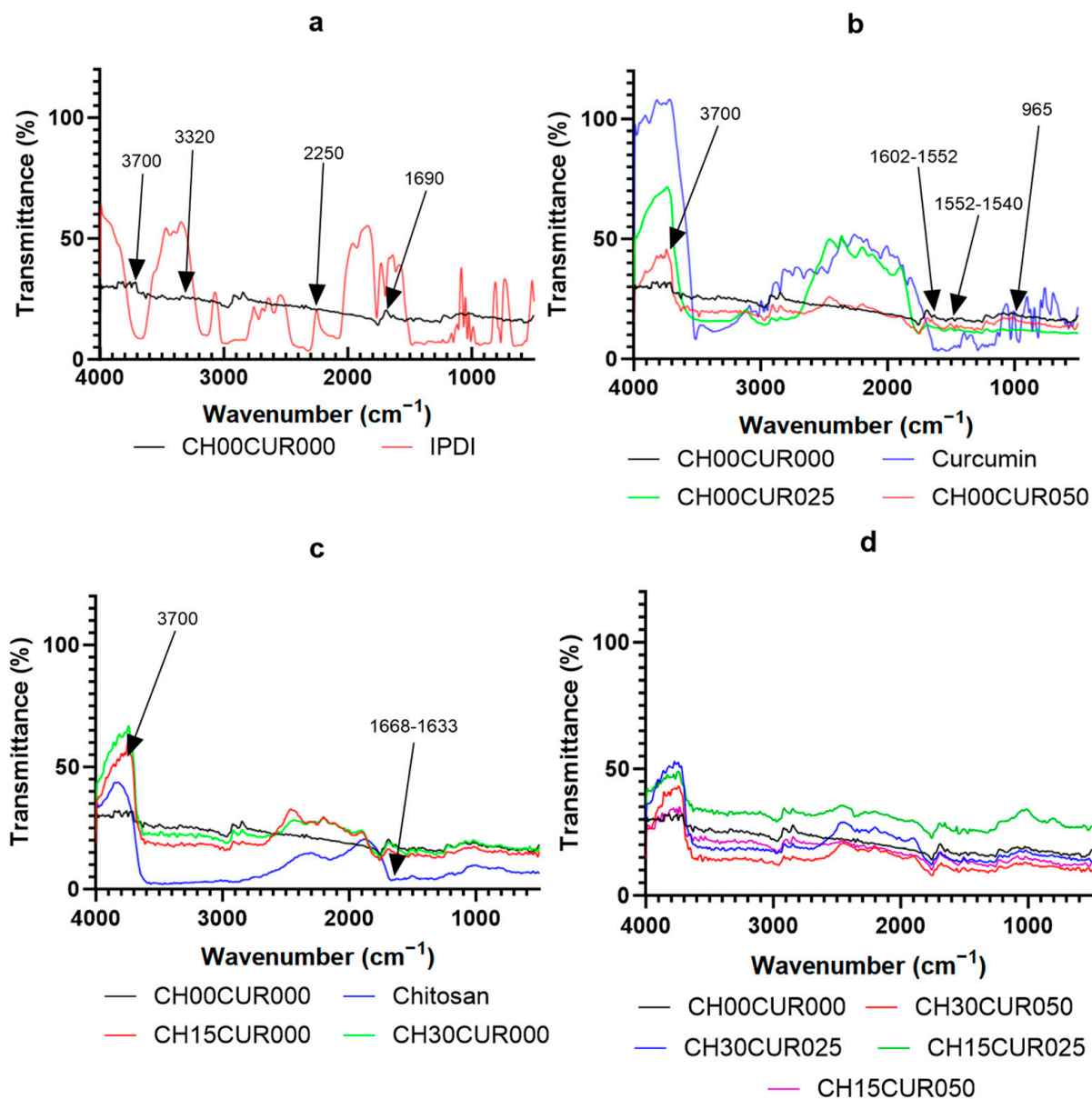
Figure 4. FTIR spectra of polyurethane formulations: (a) CH00CUR000 and isophorone diisocyanate (IPDI); (b) CH00CUR000, curcumin, CH00CUR025, CH00CUR050; (c) CH00CUR000, chitosan, CH15CUR000, CH30CUR000; (d) CH00CUR000, CH30CUR050, CH30CUR025, CH15CUR025, CH15CUR050.
