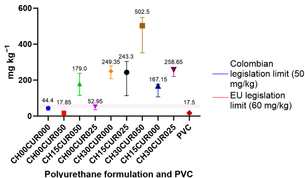
Figure 8. Median with CI 95% of overall migration of polyurethane formulations and PVC. The significantly different groups ( p < 0.05 ) were CH00CUR000-CH30CUR050, CH00CUR050-CH30CUR050 and CH30CUR050-PVC.
