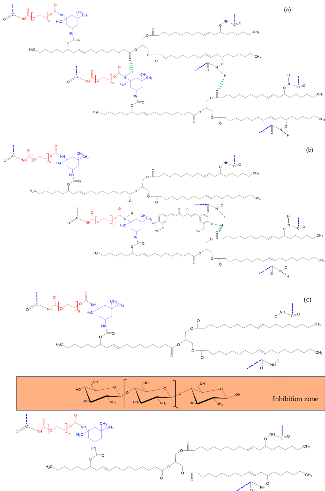
Scheme 2. Illustration of some possible hydrogen bonds formation. (a) PU-PU, (b) PU-CUR-PU, (c) PU-CH. The hydrogen bonds are represented with the green horizontal lines.
