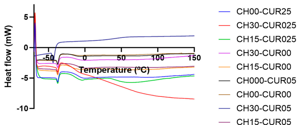
Figure 7. Differential scanning calorimetry (DSC) of polyurethane formulations.
