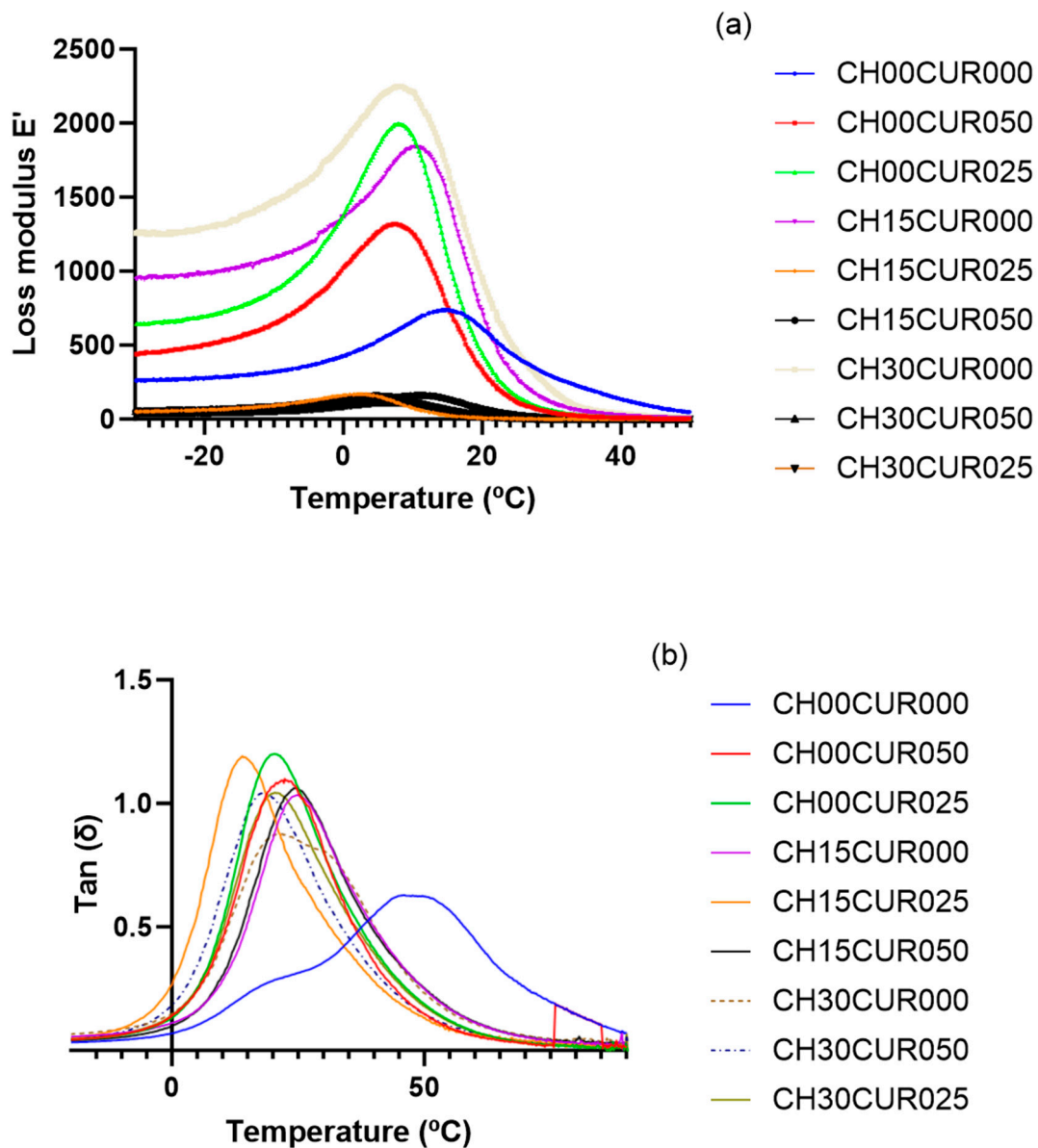
Figure 6. Dynamic mechanical thermal analysis (DMTA) of polyurethane formulations. (a) The loss modulus, (b) the \text{Tan}(\delta) .
