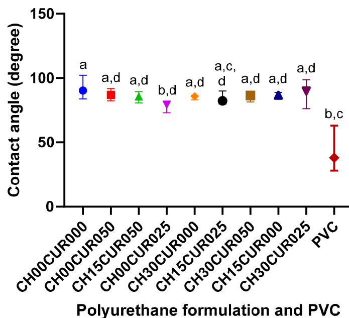
Figure 3. Contact angle of polyurethane formulations and PVC. Median with CI 95% of contact angle of polyurethane formulations and PVC. Any bar with the same letter is not significantly different ( p > 0.05 ).
