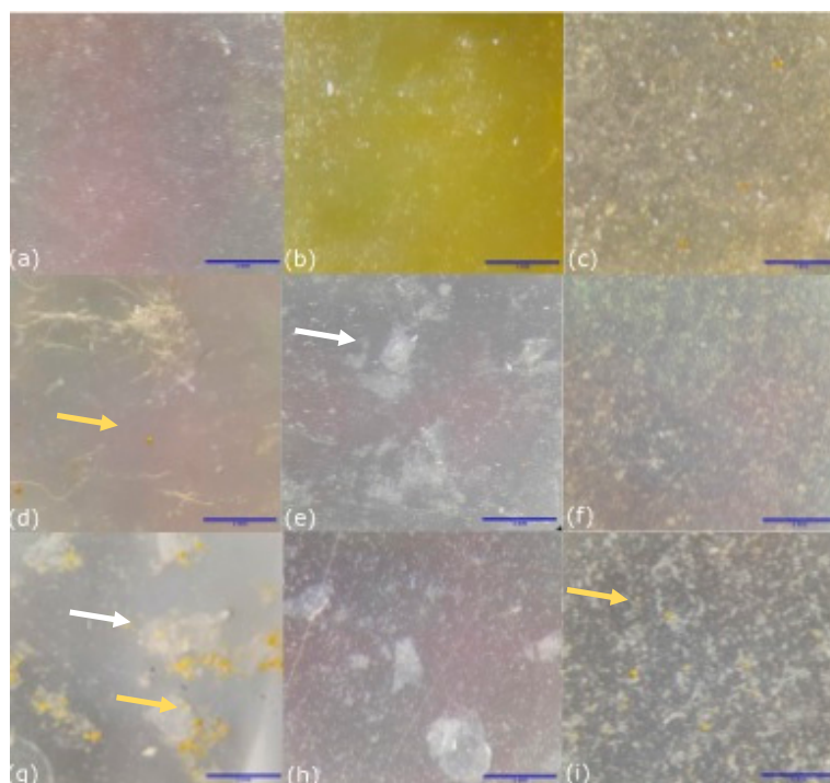
Figure 1. Stereoscope images of polyurethane formulations: (a) CH00CUR000, (b) CH00CUR050, (c) CH15CUR050, (d) CH00CUR025, (e) CH30CUR000, (f) CH15CUR025, (g) CH30CUR050, (h) CH15CUR000, and (i) CH30CUR025. The blue bar on the scale is equivalent to 1 mm. The white arrows point to chitosan, and the yellow arrows point to curcumin.
