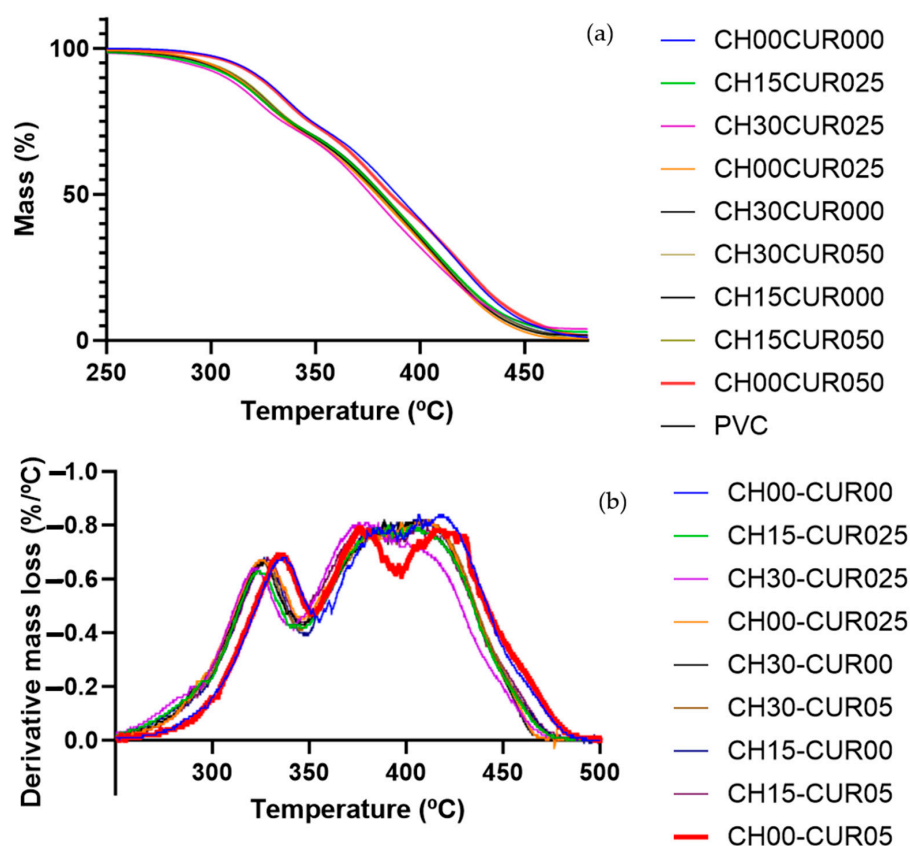
Figure 5. Thermogravimetric (TGA) (a) and derivative thermogravimetry (DGA) (b) curves of polyurethane formulations.
