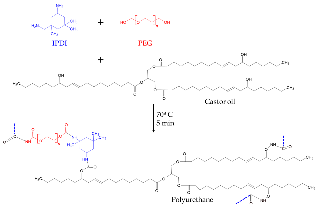
Scheme 1. Reaction scheme of the polyurethane synthesis.
