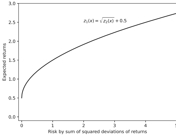
Fig. 3 The efficient frontier in the risk-returns space
