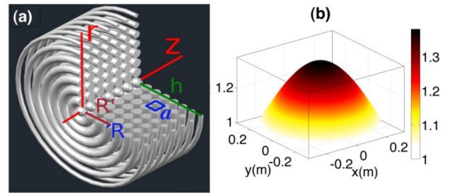
FIG. 1. (Color online) (a) Parameters used in the axisymmetric GRIN lens. (b) Axisymmetric distribution of the refraction index used in the axisymmetric GRIN lens.
