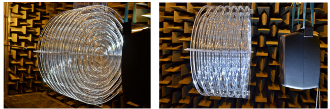
FIG. 3. (Color online) Views of the experimental set-up showing the lens-source system.
