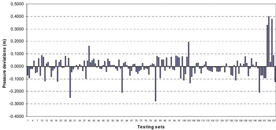
Figure 6: Comparison of EPANET and predicted ANN results for pressures - Node 90
