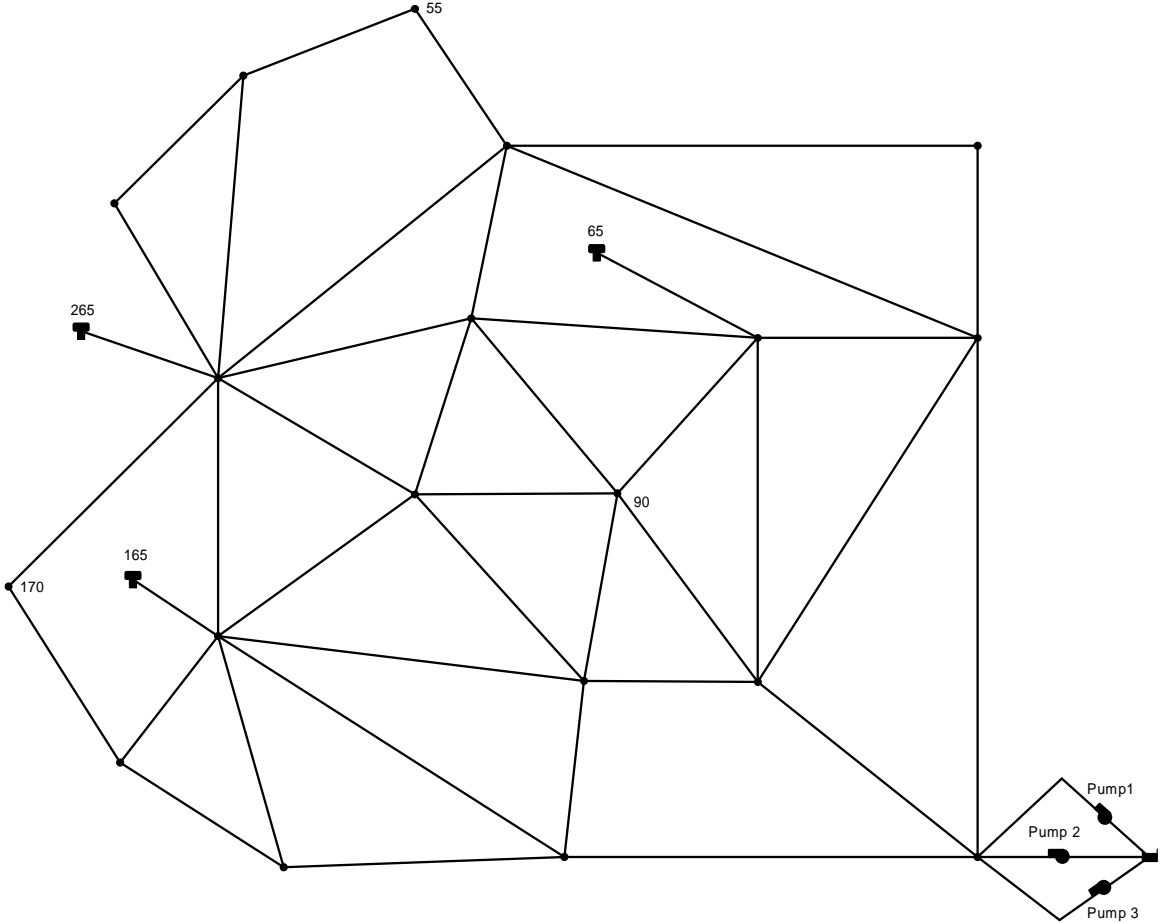
Figure 4: The Hypothetical Any Town (Modified) water-distribution network
