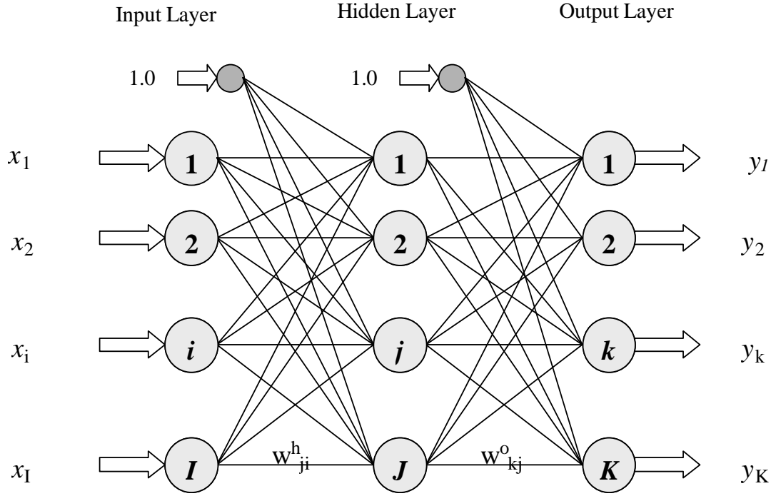
Figure 1: Architecture of an artificial neural network
