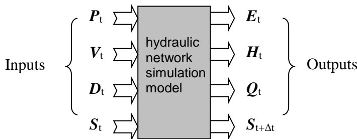
Figure 2 Input-output model of a water distribution network
