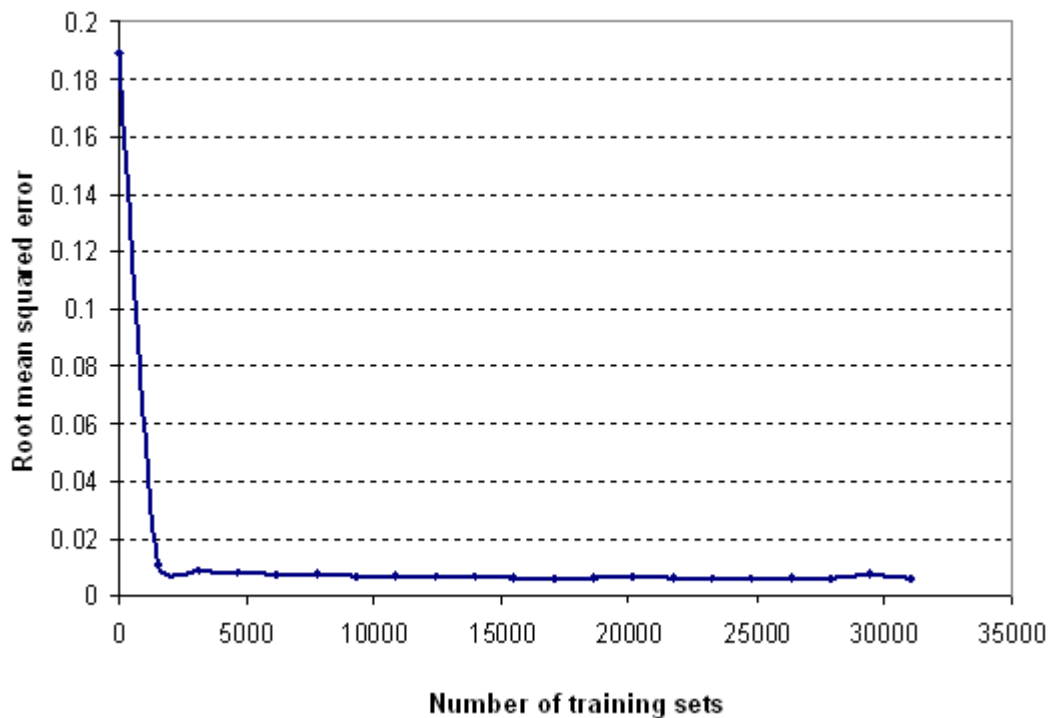
Figure 5: Relationship between RMSE and number of training sets
