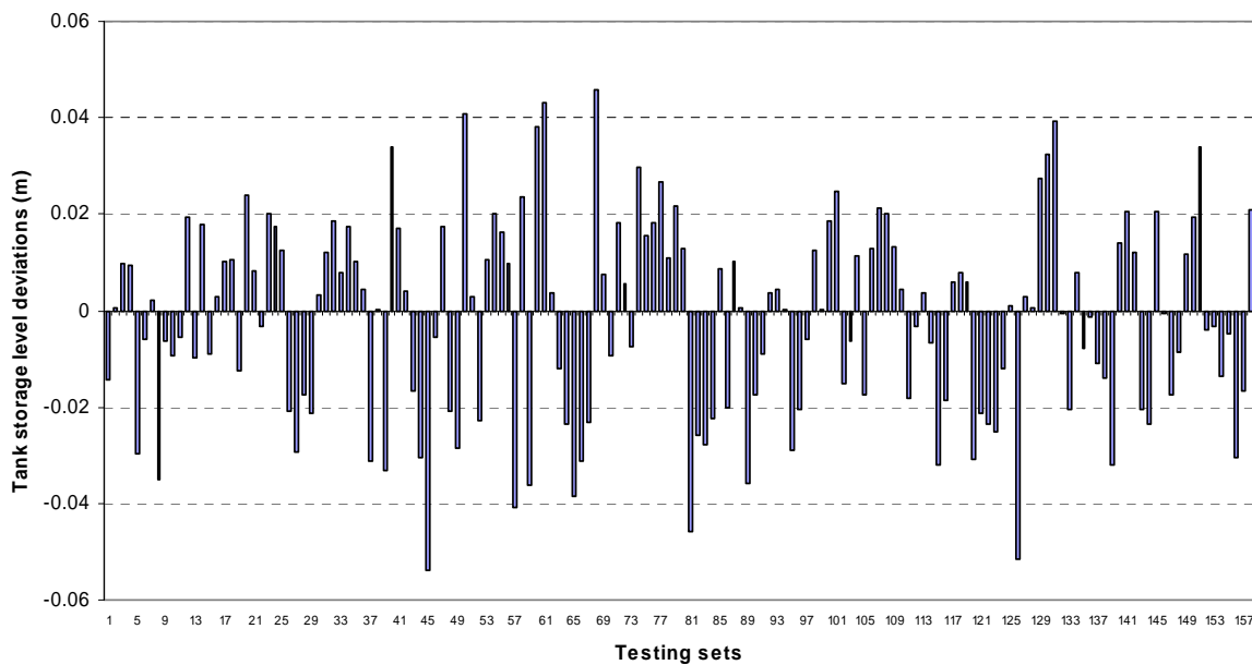
Figure 7: Comparison of EPANET and predicted ANN results for storage tank water level - Tank 65
