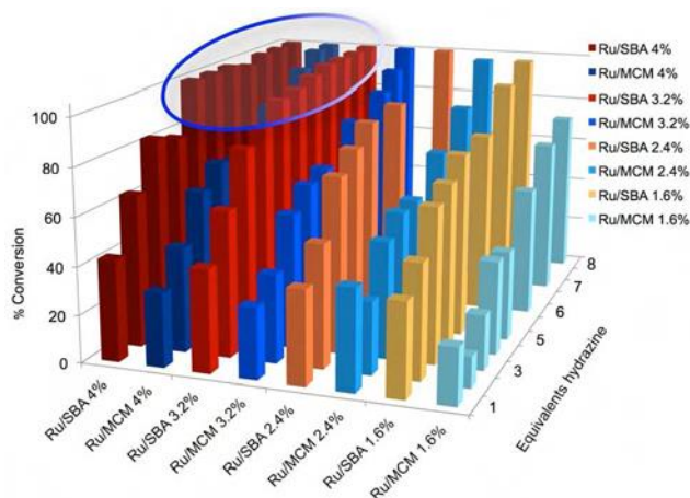
Figure 1. Conversion of nitrobenzene as a function of employed catalyst, at various mol percentages and different equivalents of hydrazine monohydrate. The oval indicates the region of near-quantitative conversion as selected from the HT data.
