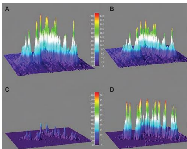
Figure 6: 3D plots of accumulated emission intensity over a catalyst surface over 25 s (A) the following 25 s (B), a difference spectrum of (A) minus (B) shown in (C) and a rescaled image of (C) at 5× the scale of (A), (B) and (C) shown in panel (D). The area displayed is 15.75 x 22.5 μm.
