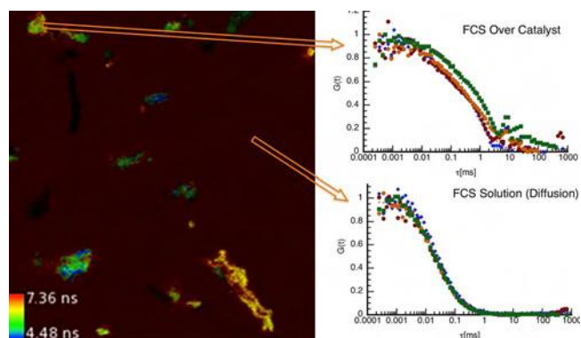
Figure 4. FLIM image acquired with 440 nm laser excitation during reduction of NN-1, where the bright spots correspond to catalyst (left). FCS curves when focused on catalyst spots (top right) and solution spots (bottom right). Solution spots measured after some accumulation of the product AN-2.
