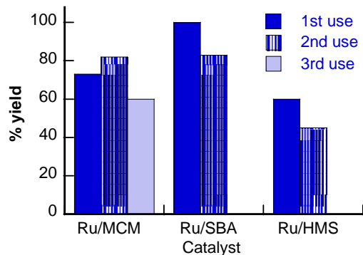
Figure 2. Percentage of the reusability of the materials studied for the reduction of nitrobenzene under the optimized reaction conditions.
