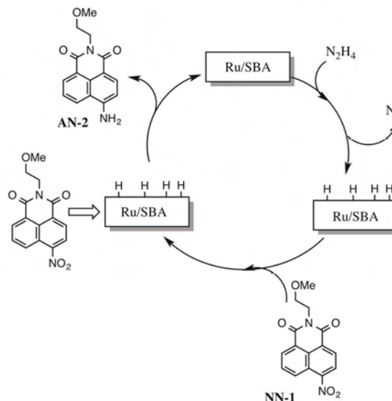
Scheme 2. Proposed mechanism for the Ru@SBA catalyzed reduction of nitro compounds to amines, illustrated for the example of NN-1.
