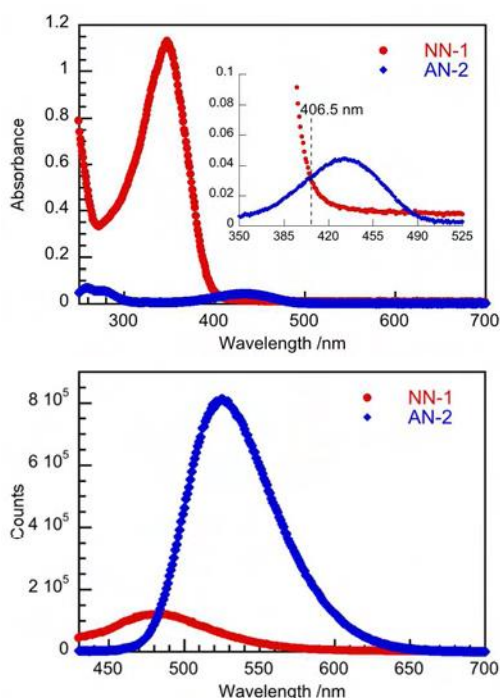
Figure 3. Absorbance spectra of NN-1 and AN-2 (after reaction), top, as well as (bottom) emission spectra of for both compounds (with matched absorbance and excitation at 406.5 nm – see SI).
