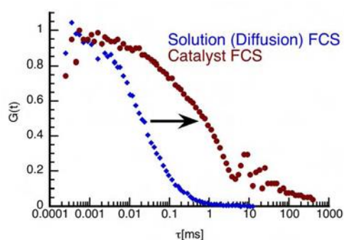
Figure 5. Representative FCS curves with 440 nm excitation when excitation/image acquisition is focused on either a catalyst (red) or solution (blue) spot.
