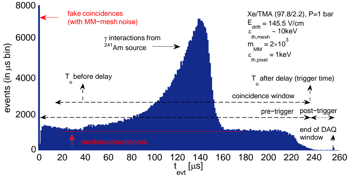
Figure 2. Distribution of event times registered at NEXT-MM when triggering in coincidence with \alpha 's from a ^{241}\text{Am} source, detected in an auxiliary Si-diode. The observed exponential shape is dominated by the mean free path of the 59.5 keV \gamma emitted in the decay of ^{237}\text{Np} to its ground state, modulated by solid angle and other geometrical effects. The edges of the TPC cathode and the readout plane are clearly discernible over a flat background. The chosen settings reflect typical working conditions described in the text.
