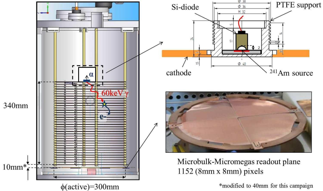
Figure 1. Experimental setup used for the characterization of NEX-T-MM with low energy \gamma photons, under a Xe/TMA mixture. Left: transverse section of NEX-T-MM showing the field cage, source position and readout plane. Right-up: close-up of the ^{241}\text{Am} source in its PTFE enclosure. Right-down: photo of the readout plane, showing the arrangement in 4 separate quadrants.
