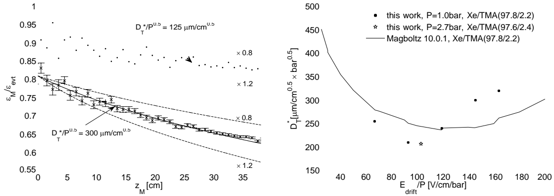
Figure 13. Left: behaviour of the highest charge fraction contained in a single pixel \varepsilon_M / \varepsilon_{evt} as a function of the z -position of the deposit for E_{drift}/P = 145.5 V/cm/bar at P = 1 bar (crosses) and E_{drift}/P = 103.6 V/cm/bar at P = 2.7 bar (points). The transverse diffusion coefficients extracted from the fit proposed in the text are indicated together with the trends for 20% variations around it, to illustrate the sensitivity of the method. Right: transverse diffusion coefficient obtained from this analysis including statistical uncertainties only. Systematic effects related to the naive treatment of the initial ionization cloud have not been evaluated.
