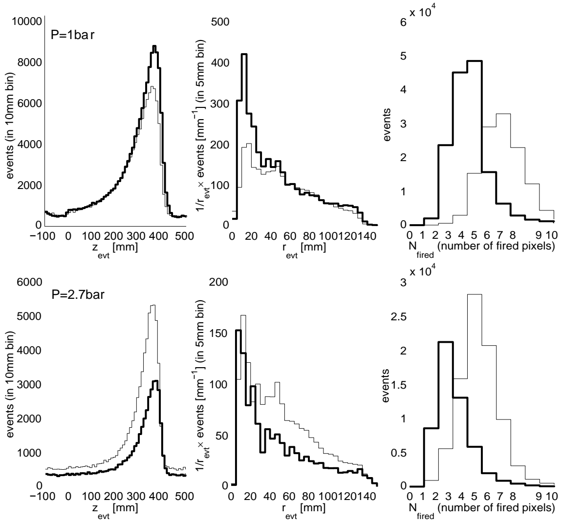
Figure 5. Spatial characteristics of the ionization created in the TPC by \gamma -rays produced by a ^{241}\text{Am} source placed at the TPC cathode ( D = 38 cm). Two energy regions have been selected after calibration ( 20 \text{ keV} < \varepsilon_{\text{evt}} < 40 \text{ keV} and 50 \text{ keV} < \varepsilon_{\text{evt}} < 70 \text{ keV} ) corresponding to the \sim 30 \text{ keV} Xenon escape peak (thick line) and the full-absorption 59.5 \text{ keV} one (thin line). Left: distribution along the drift region. Middle: radial distribution. Right: pixel multiplicity.
