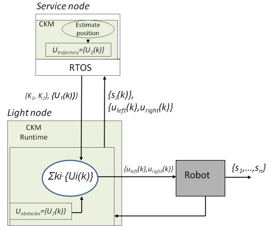
Figure 7: Control structure. Experiment 2
