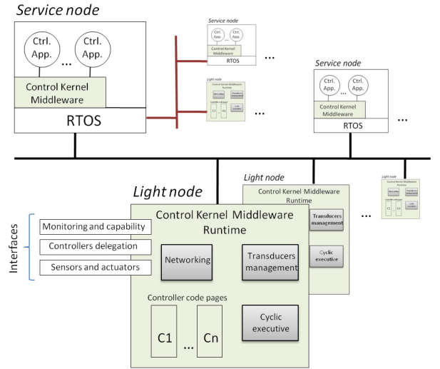
Figure 2: Control Kernel based architecture.
