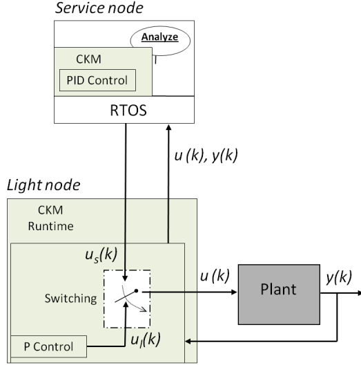
Figure 5: Control structure. Experiment 1
