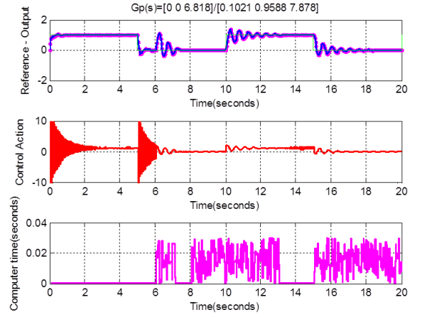
Figure 6: Switching control due to interferences.
