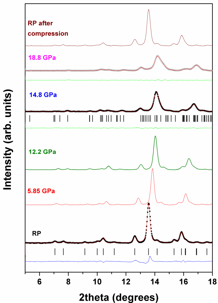
Figure 2. Powder XRD patterns of tetragonal \text{Sr}_2\text{ZnGe}_2\text{O}_7 at some representative pressure. Fitted profiles for the XRD data at RP, 14.8 and 18.8 GPa are shown. The Bragg peak positions are shown as ticks and difference plots as continuous line below fitted profiles.
