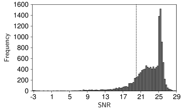
Figure 3. SNR histogram for the reconstructed words of tst and trn sets. The dashed vertical line indicates 20 dB. The mean SNR value is 22.8 \text{ dB} \pm 3.6 .
