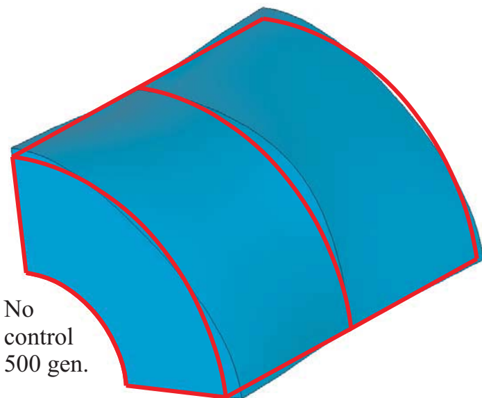
Fig. 13. 3D model. Evolutionary algorithm + Ansys®. Influence of \gamma over the optimal solution found and comparison with optimal analytical solution (red contour).
