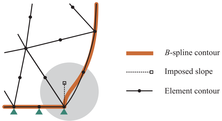
Fig. 6. Geometrical constrain and mesh.
