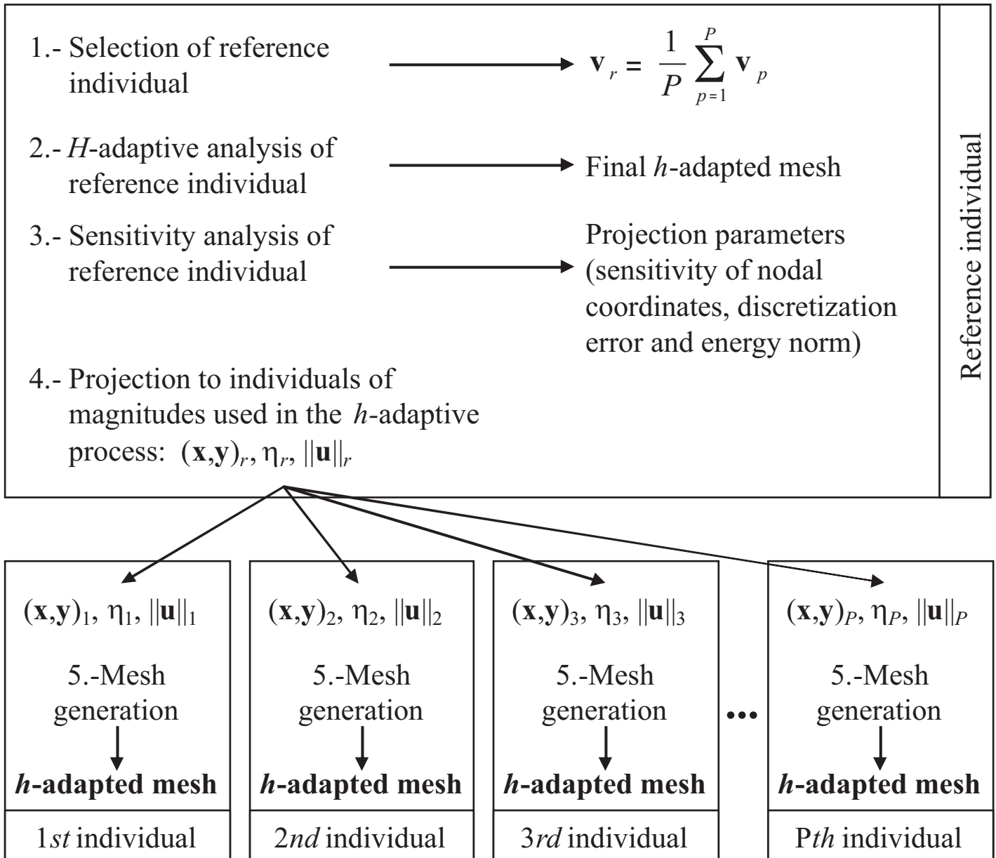
Fig. 15. Algorithm for the direct definition of h -adapted meshes for all the individuals of a generation.
