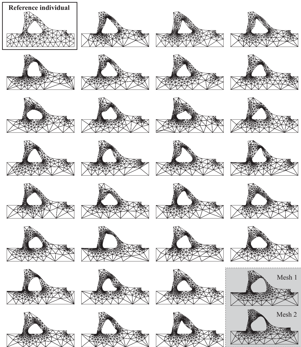
Fig. 22. Gravity dam. Generation of FE meshes for a generation of individuals by projection from a reference individual. Only the highlighted individual required remeshing.
