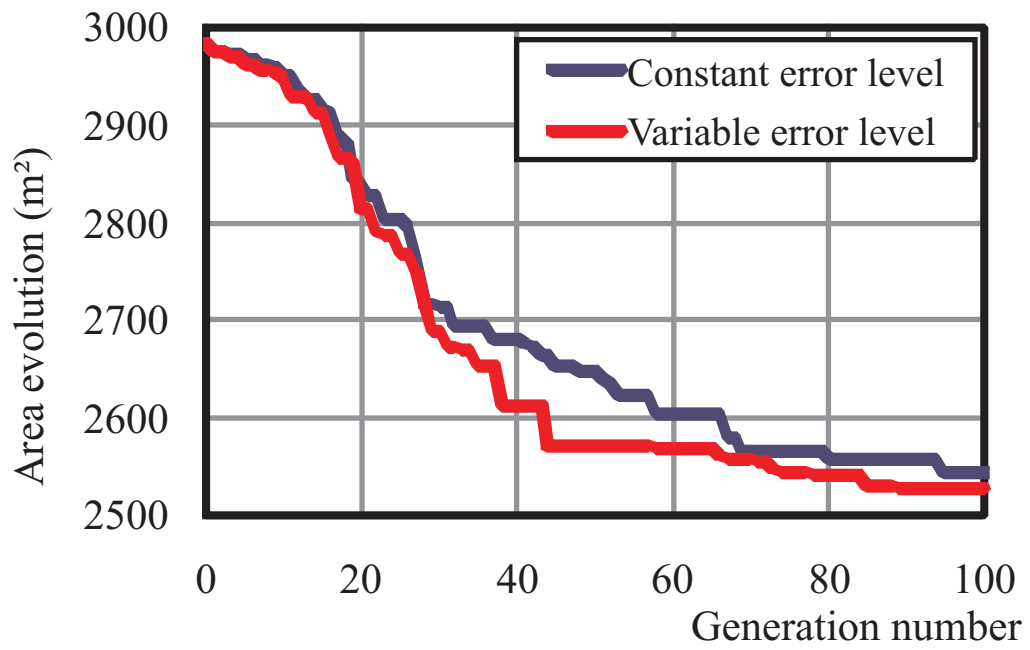
Fig. 24. Gravity dam. Area evolution.
