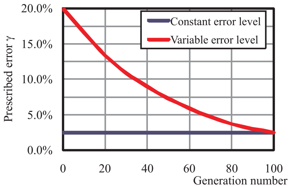
Fig. 23. Gravity dam. Evolution of the prescribed error \gamma .
