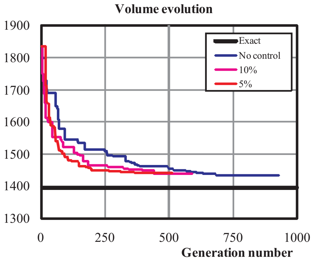
Fig. 11. 3D model. Evolutionary algorithm + Ansys®. Influence of \gamma over the evolution of the objective function (volume).
