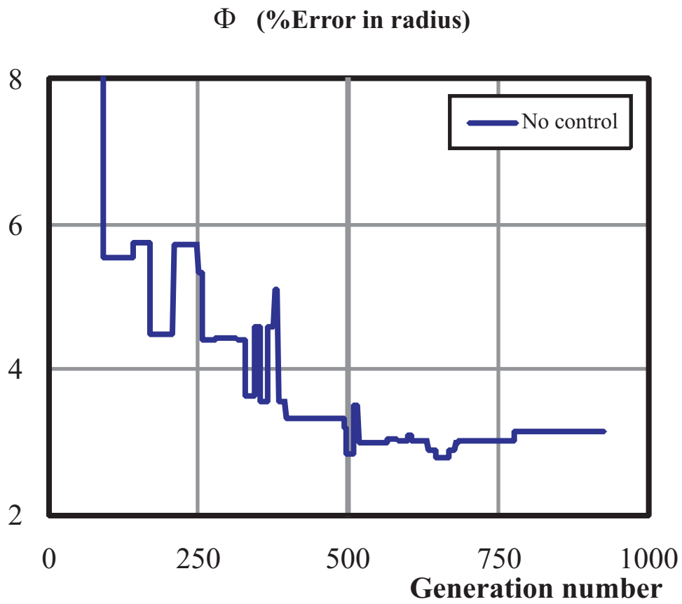
Fig. 14. 3D model. Evolutionary algorithm + Ansys®. Evolution of \Phi with no error control.
