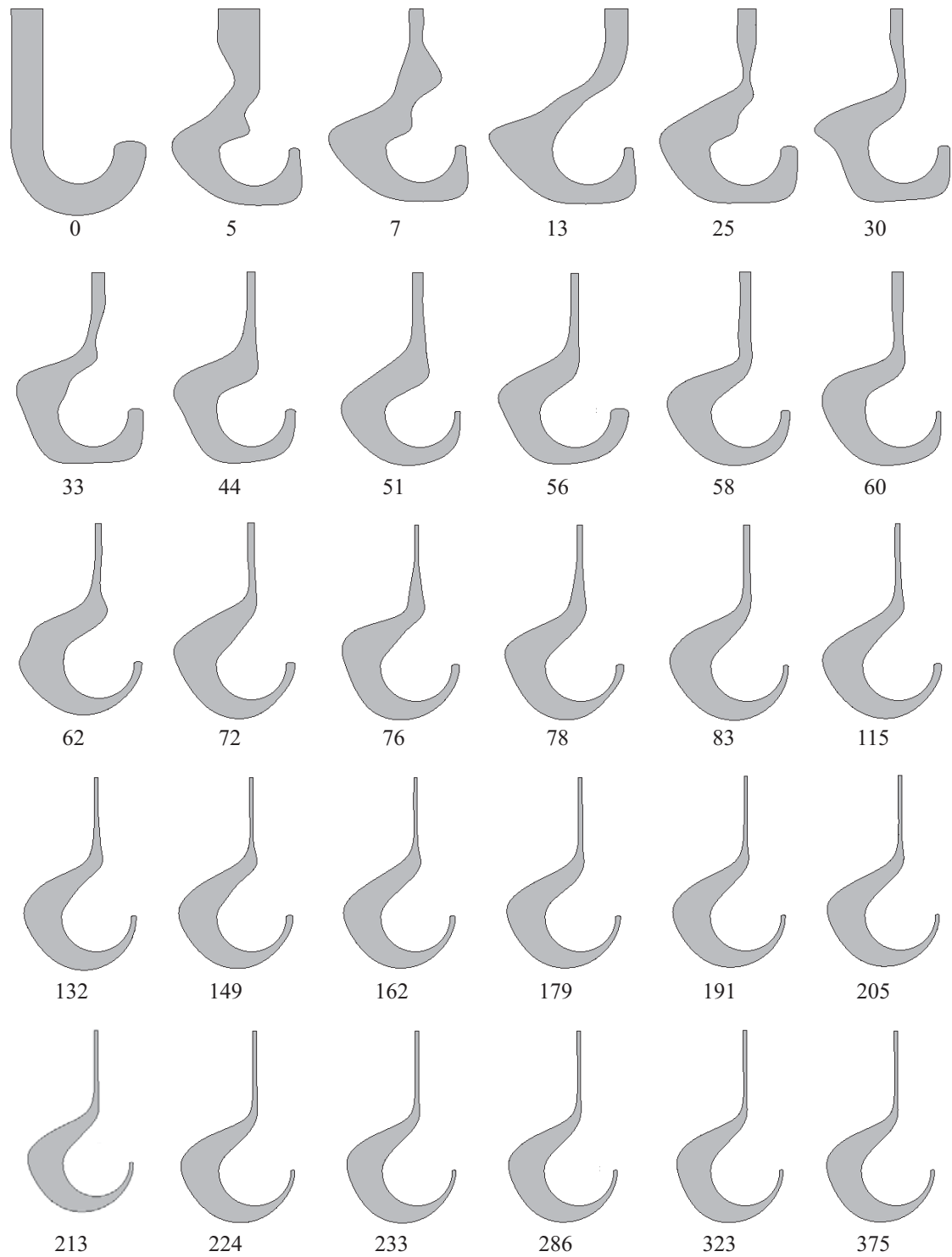
Fig. 19. Hook. Evolution of the best individual during the optimization process. The figure below each geometry indicates the generation number where the geometry was created.
