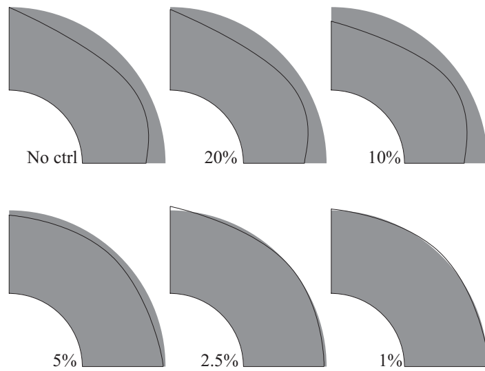
Fig. 5. 2D model. Evolutionary algorithm. Influence of \gamma over the optimal solution found (black contour) and comparison with optimal analytical solution (shaded area).
