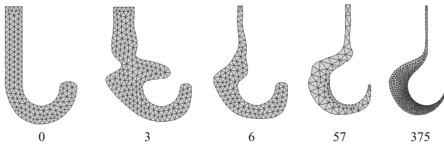
Fig. 18. Hook. Mesh densities used along the optimization process. The geometries represented correspond to a representative individual of a selection of generations.
