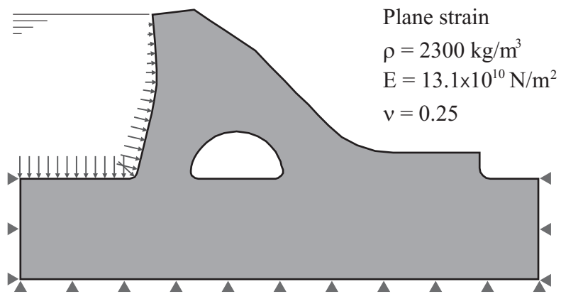
Fig. 20. Gravity dam. Analysis model.
