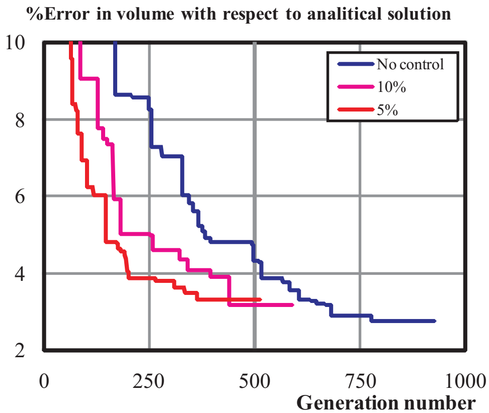
Fig. 12. 3D model. Evolutionary algorithm + Ansys®. Influence of \gamma over the evolution of the error in the objective function with respect to the optimal analytical solution.
