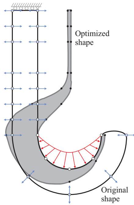
Fig. 16. Hook optimization. Original shape and design variables. Optimized shape.
