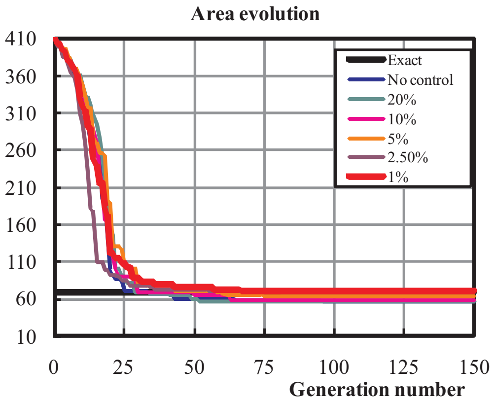
Fig. 3. 2D model. Evolutionary algorithm. Influence of \gamma over the evolution of the objective function.
