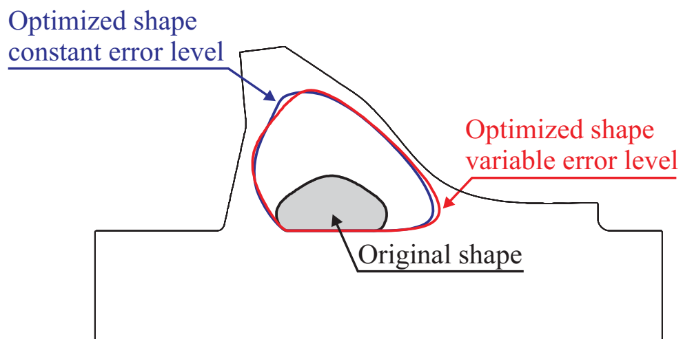
Fig. 25. Gravity dam. Optimized geometries versus original geometry.
