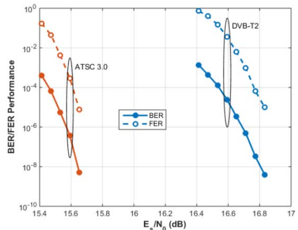
Fig. 10. Comparison of BER/FER performance for ATSC 3.0 and DVB-T2. LDPC codeword size 64800 bits with code rate 9/15, modulation 256QAM.
