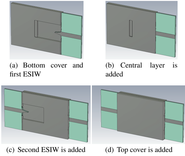
Fig. 2 Schematic 3D views of the stacked ESIW transition, with the assembling procedure of the 5 layers. (a) Bottom cover and first ESIW line. (b) Central layer is added. (c) Second ESIW is added. (d) Top cover is added and the assembling is completed
