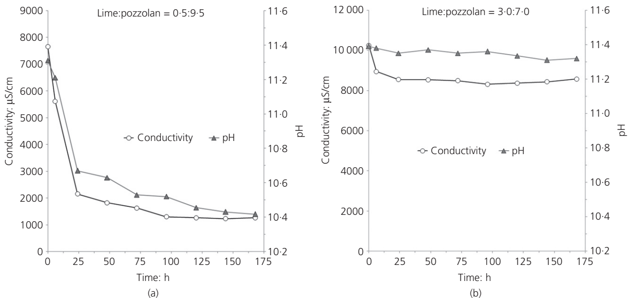
Figure 3. Electrical conductivity measurements and pH values for lime:pozzolan suspensions of: (a) 0.5:9.5 and (b) 3.0:7.0
