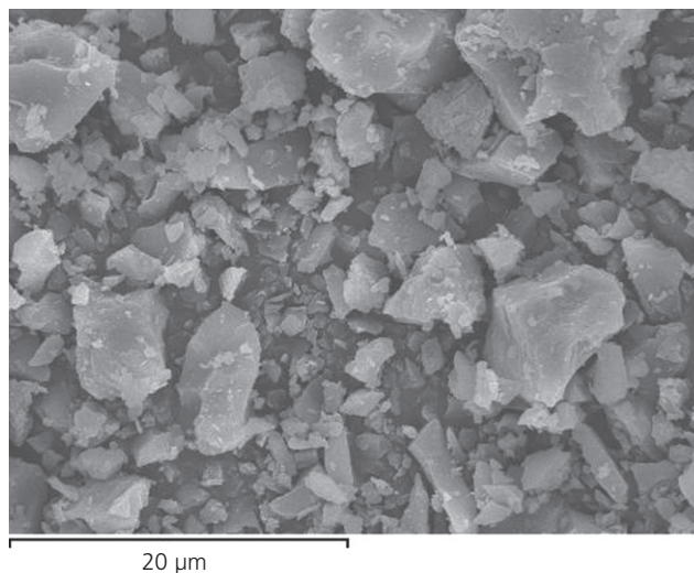
Figure 1. SEM micrograph of ground TCW
