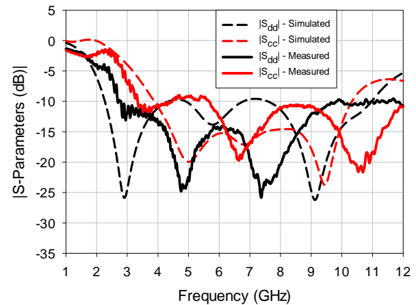
Fig. 12. Simulated and measured reflection coefficient for differential feeding ( |S_{dgl}| ) and common feeding ( |S_{cc}| ).
