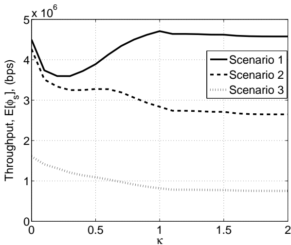
Fig. 6. Throughput achieved by users associated to the SAP as a function of \kappa for different backhaul scenarios.
