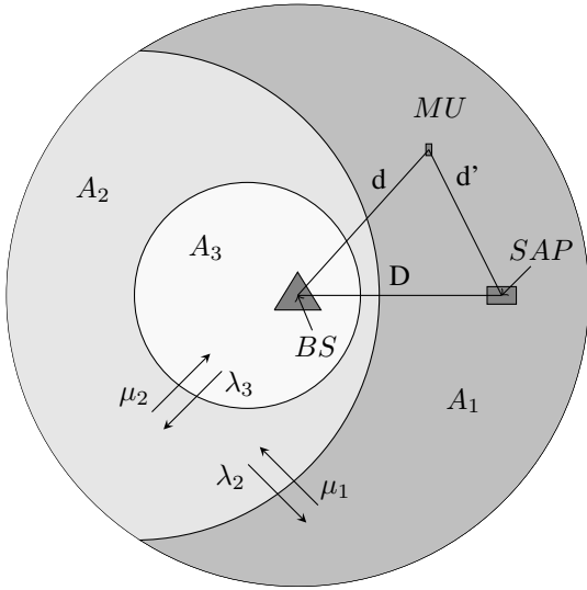
Fig. 1. Different interference regions, K = 3 .
