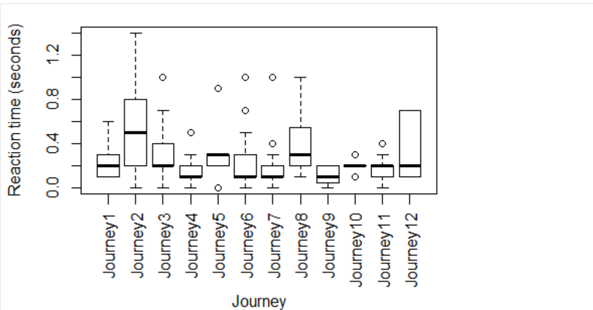
Figure 5-Drivers' reaction time.
