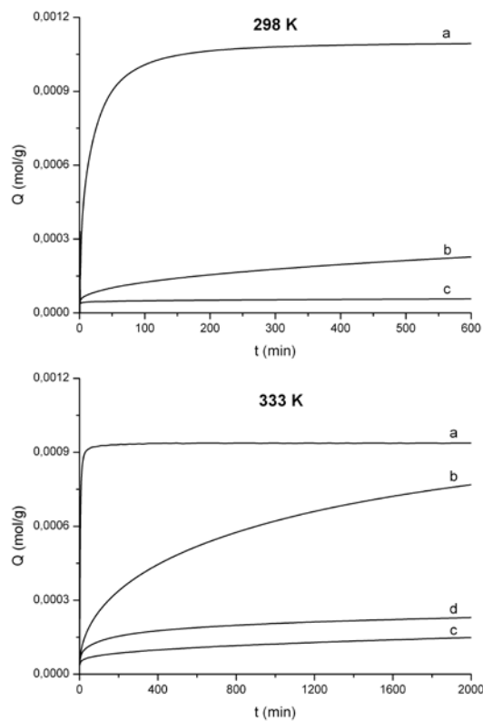
Figure 1. Adsorption kinetics of C 4 hydrocarbons at 298 and 333 K and 30.4 KPa in ITQ-32. trans-2-butene (a), 1-butene, (b), butane (c) and cis-2-butene (d).
