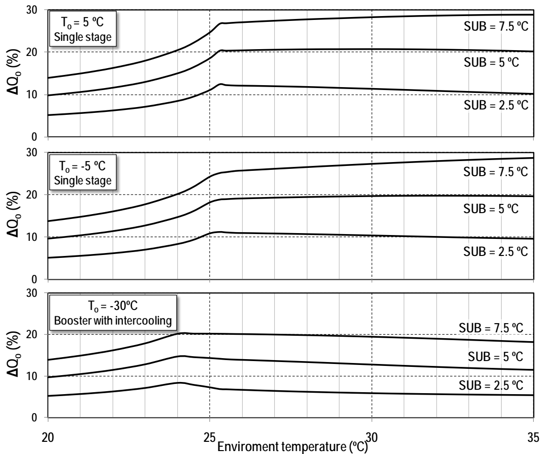
Figure 11. Percentage increment of cooling capacity versus the transcritical system for different subcooling degrees
