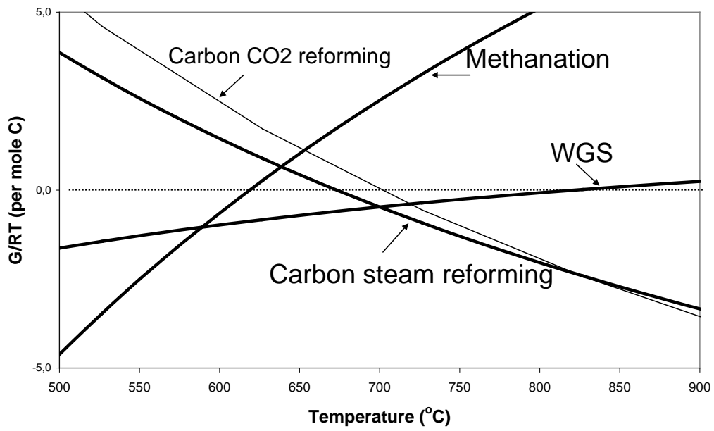
Figure 1 – Gibbs Free energy for several reactions vs. temperature.
