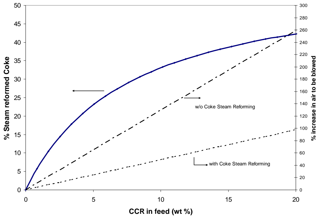
Figure 3 – Fraction of Coke to be Steam Reformed vs. Conradson Carbon in feed. Comparison of increase in air blower capacity with and w/o Steam reforming.
