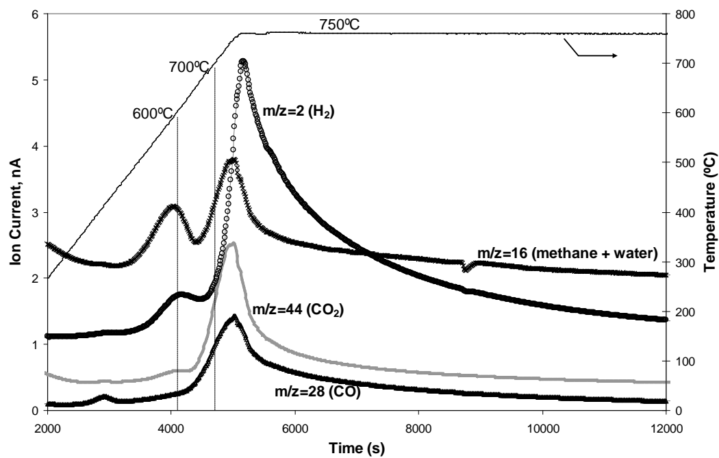
Figure 9 – m/z signals obtained from the processing of a coked sample in the presence of water in a TPD-MS unit. Hydrotalcite sample coked with VGO. m/z at 2 and 44 are shifted 0.3 and 1 nA respectively.
