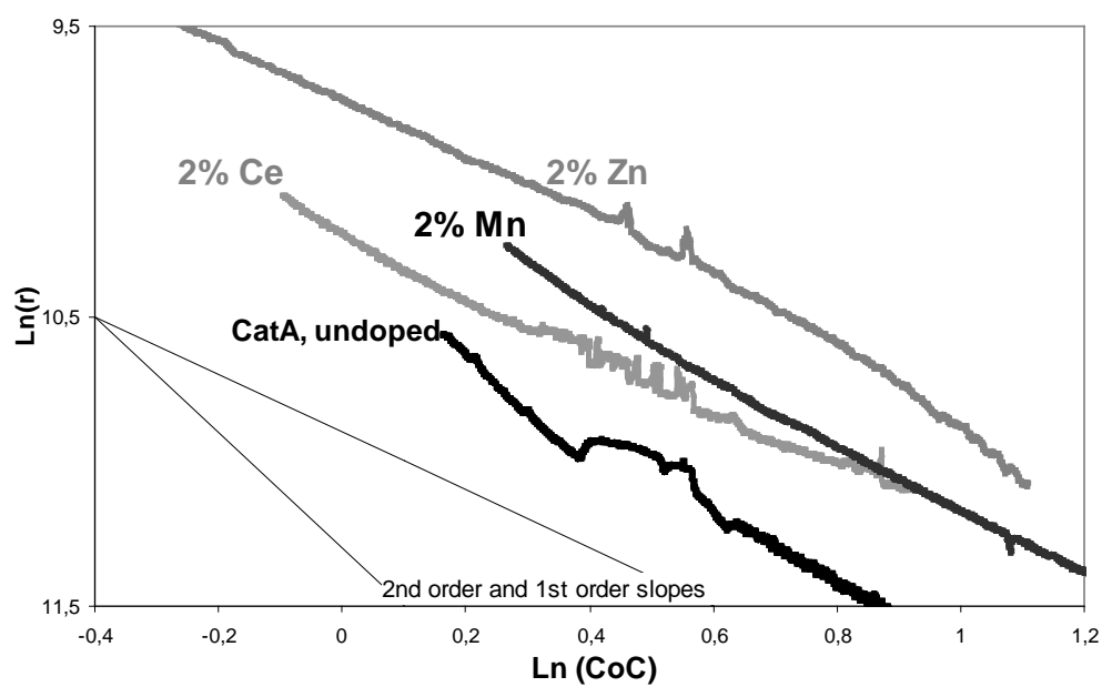
Figure 8 – Plot of kinetic data: Log of Reaction rate (in coke-on-catalyst percent per second) vs Log of CoC (in percent on catalyst), determined through TPD experiments for Metal impregnated Ecat.
