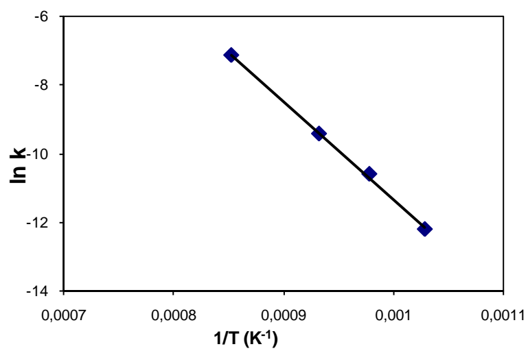
Figure 7 - Temperature dependence of rate constant
