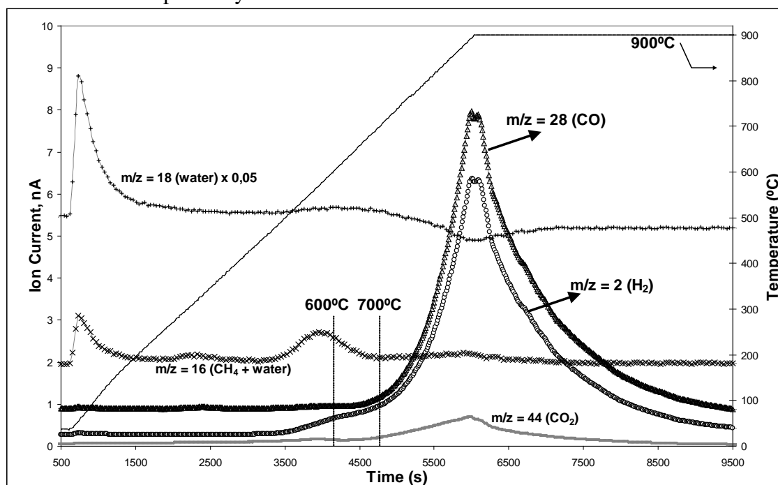
Figure 4 – m/z signals obtained from the processing of a coked sample in the presence of water in a TPD-MS unit. Ecat samples coked with VGO. m/z at 2 and 28 are shifted 0.3 and 0.8 nA respectively.
