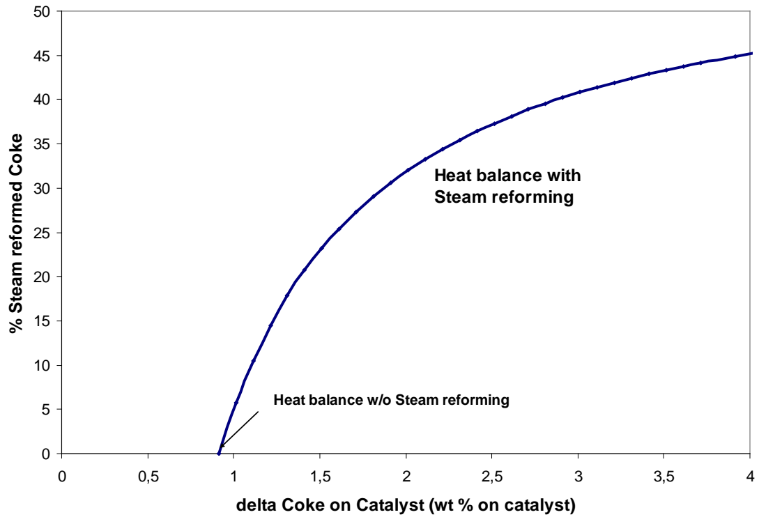
Figure 2 – Relation between the fraction of coke to be Steam Reformed with increasing coke on catalyst to maintain heat balance in the FCC regenerator. Calculations are made assuming catalyst inlet temperature of 500°C and regenerator temperature of 730°C, with vapor and steam entering at 200°C in the regenerator.
