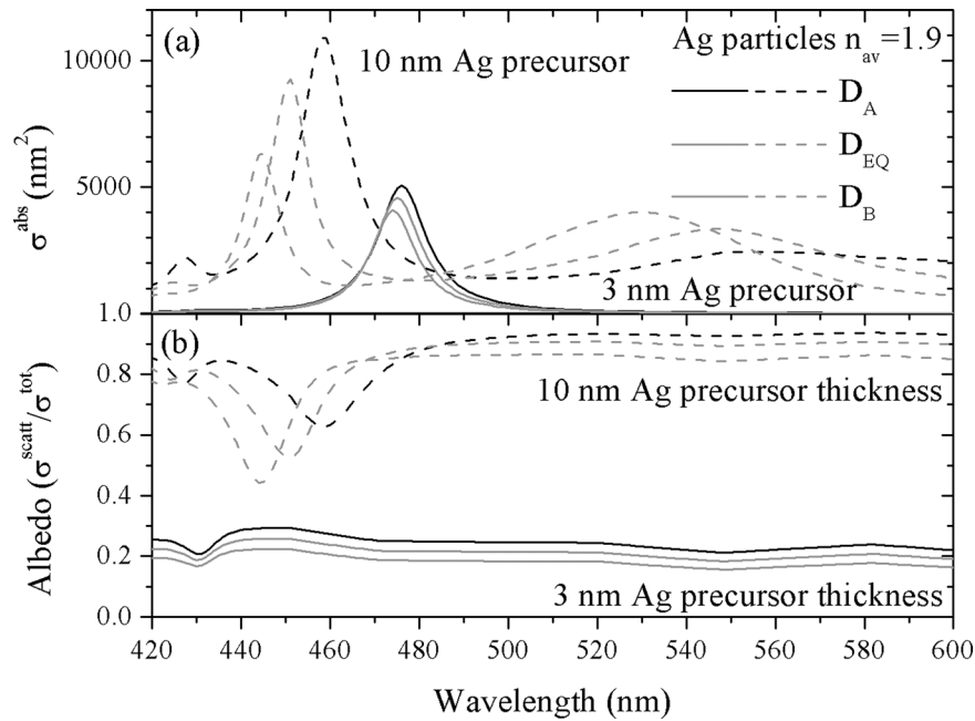
FIG. 3. (a) Simulated absorption cross section and (b) and simulated albedo. In both cases, a spherical shape has been assumed for Ag MNPs and the different diameters shown in Table II. A symmetric environment has been assumed with an averaged refractive index to take into account the higher index Si substrate.
