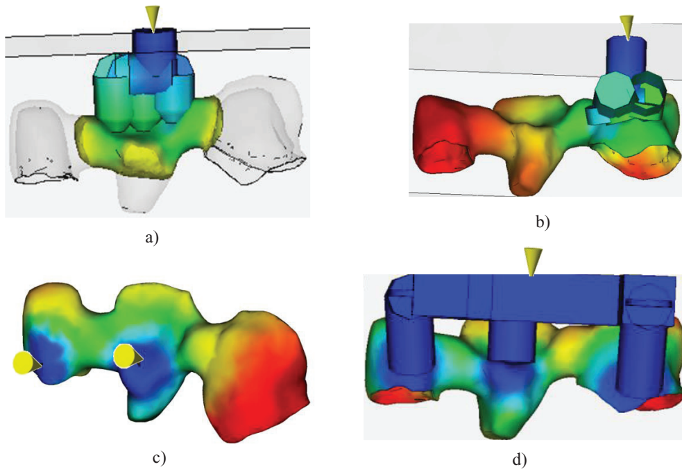
Fig. 5. (a) cluster of gates on solid piece; (b) cluster of gates on one crown; (c) one point on solid piece and on one crown; (d) one gate on solid piece and one gate on each crown.
