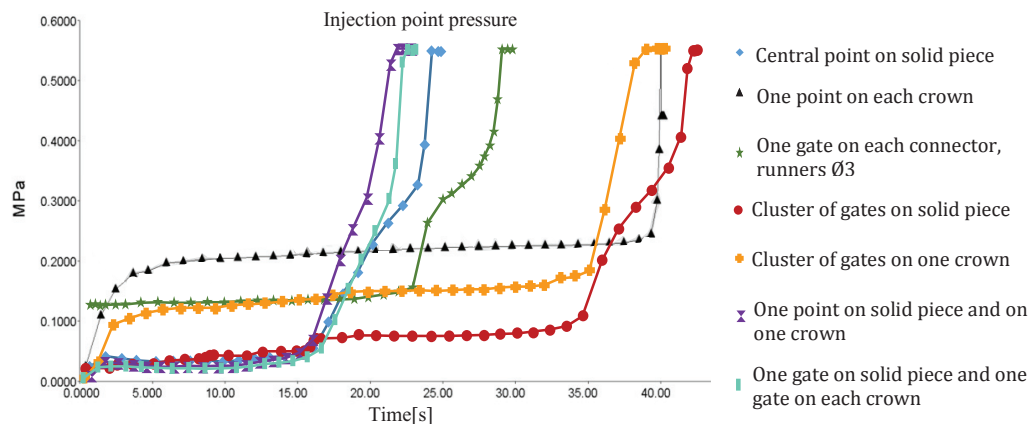
Fig. 6. Stress/time curve.
