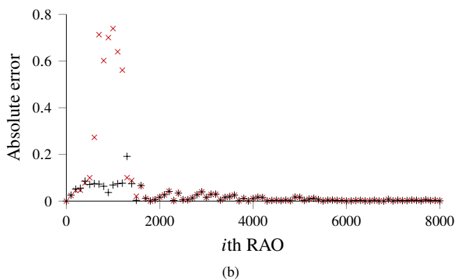
Figure 11. (a) Comparison and (b) absolute error of the expected number of successful accesses at each RAO, \mathbb{E}[M_S(i)] , obtained by simulation, by the extended reference model and by our model; a static ACB is implemented with p_{acb} = 0.5 and t_{acb} = 4 .
