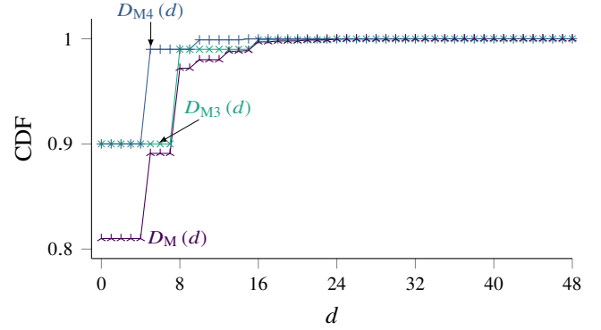
Figure 8. CDF of the access delay due to the transmission of Msg3 and Msg4 for the given probability of error during transmission, p_{\mathcal{E}_{M3}} = p_{\mathcal{E}_{M4}} = 0.1 ; the RTT of Msg3 is 8 subframes and the the RTT of Msg4 is 5 subframes.
