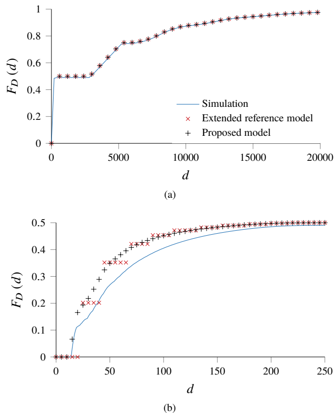
Figure 12. (a) Overall view and (b) first 250 subframes of the CDF of the access delay, F_D(d) , obtained by simulation, by the extended reference model and by our model; a static ACB is implemented with p_{\text{acb}} = 0.5 and t_{\text{acb}} = 4 .
