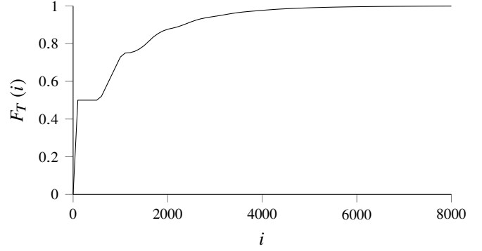
Figure 1. CDF of the barring time, given p_{\text{acb}} = 0.5 , t_{\text{acb}} = 4 s and p_{\mathcal{E}_{\text{ACB}}} = 10^{-5} .
