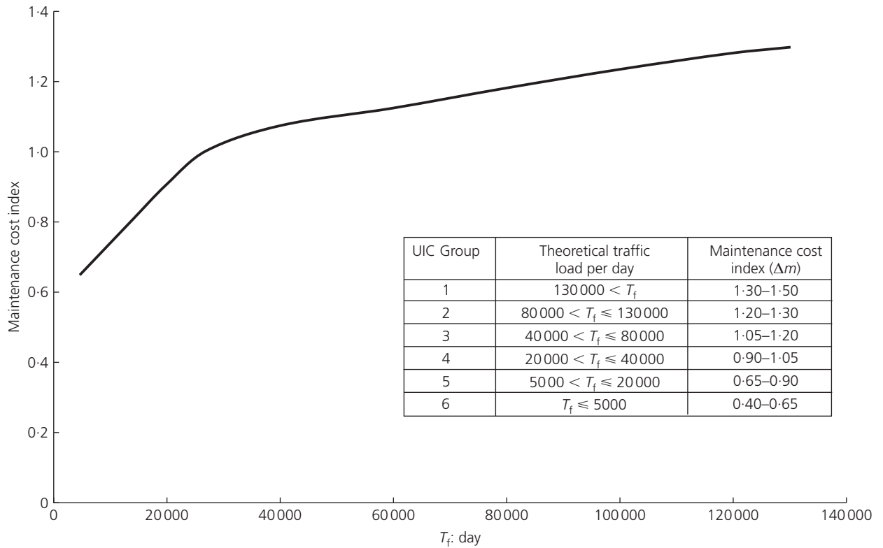
Figure 6. Variation of annual maintenance cost with the theoretical traffic load. Source: own source, based on UIC (1992)
