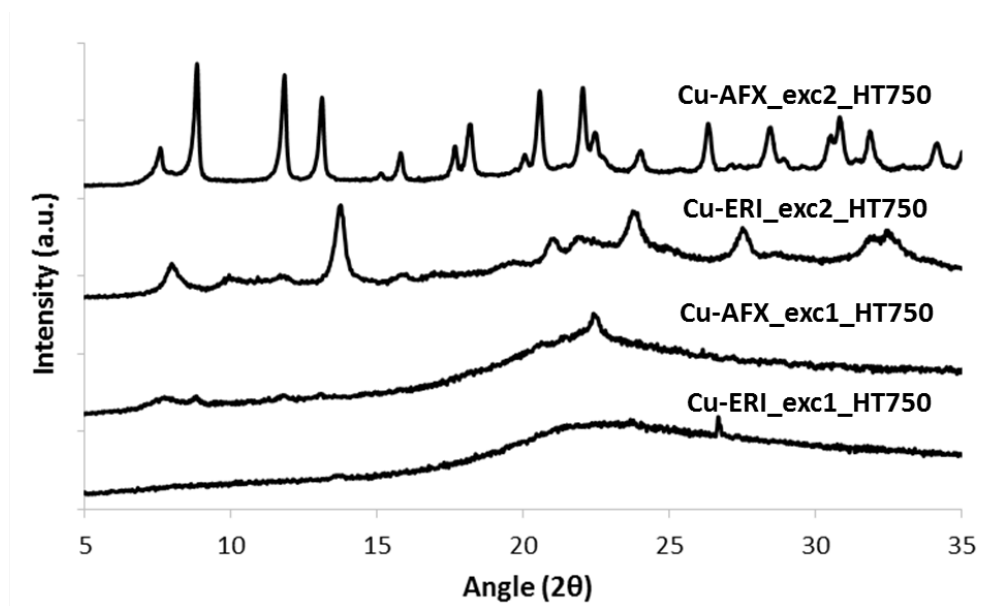
Figure 10: PXRD patterns of the Cu-exchanged ERI and AFX samples after steaming at 750°C for 13 hours
