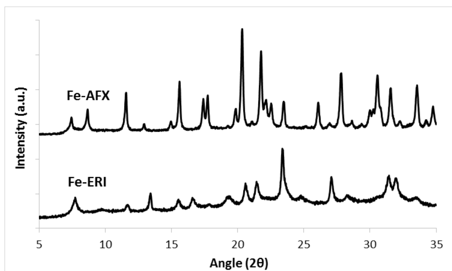
Figure 11: PXRD patterns of the as-prepared one-pot synthesized Fe-containing ERI and AFX samples
