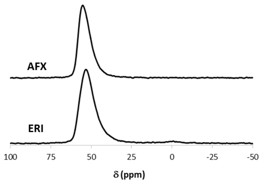
Figure 6: ^{27}\text{Al} MAS NMR spectra of the as-prepared ERI and AFX samples
