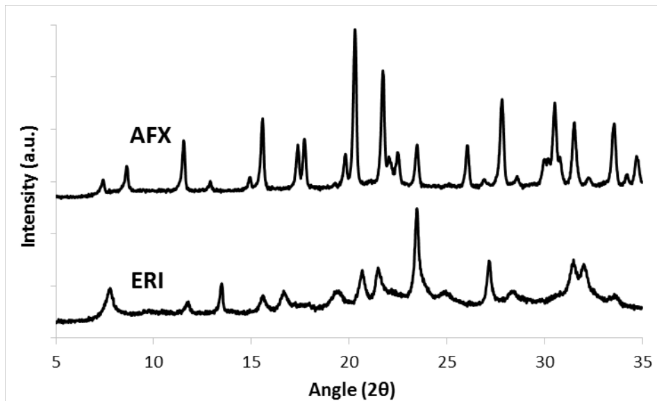
Figure 5: PXRD patterns of the as-prepared ERI and AFX samples
