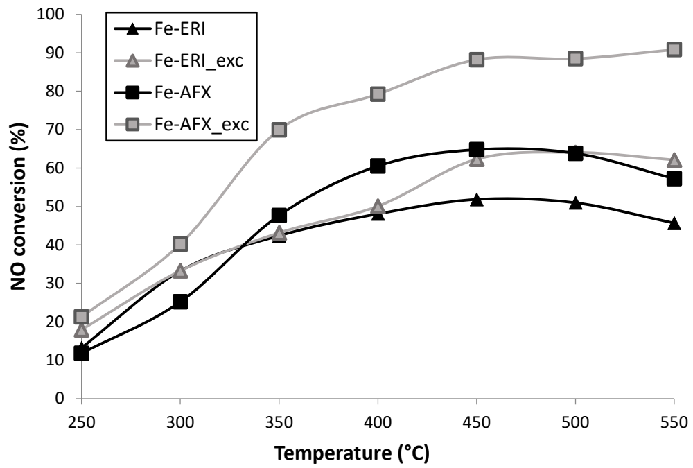
Figure 13: Measured NO conversion over iron-containing ERI and AFX materials in the NH 3 -SCR reaction
