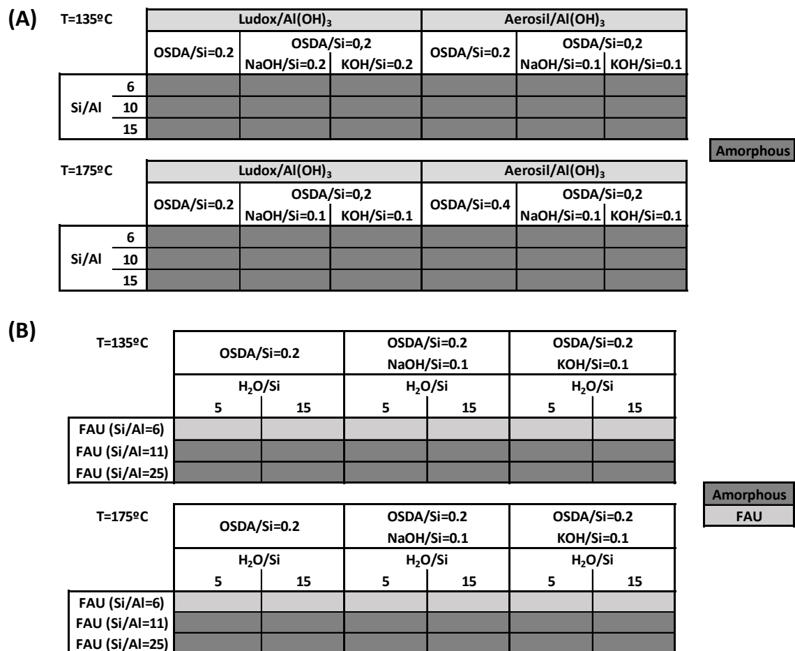
Figure 3: Phase diagrams achieved when using OSDA-1 with Ludox/Aerosil and Al(OH) 3 as silicon and aluminum sources (A) or commercially available FAU zeolites (B)
