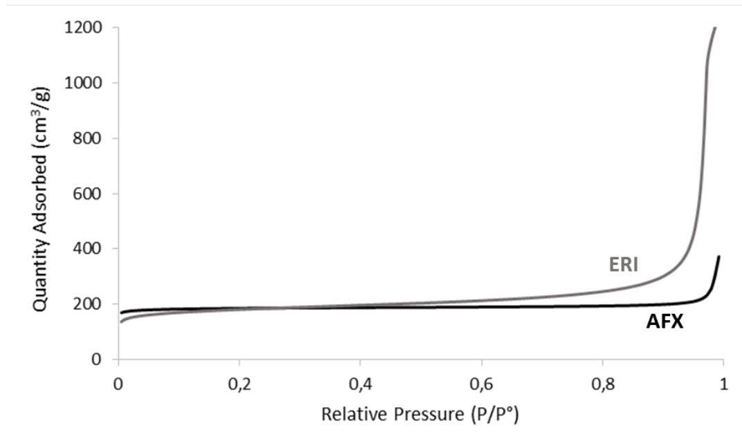
Figure 8: N 2 adsorption isotherms for the calcined ERI and AFX zeolites
