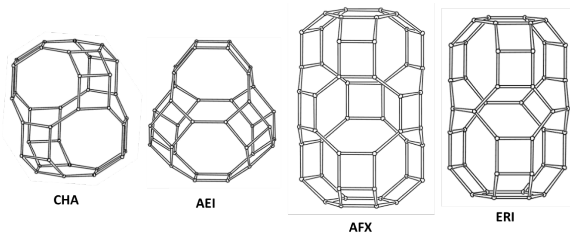
Figure 1: Cavities present within the structure of different small pore zeolites
