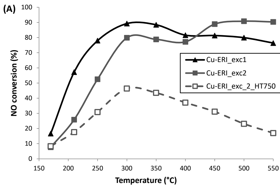
Figure 9: Measured NO conversion over copper-containing ERI-related (A) and AFX-related (B) materials in the NH 3 -SCR reaction.
