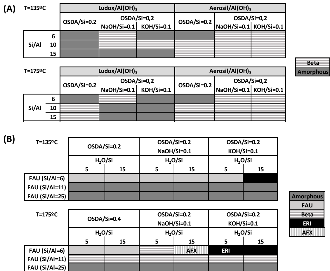
Figure 4: Phase diagrams achieved when using OSDA-2 with Ludox/Aerosil and Al(OH) 3 as silicon and aluminum sources (A) or commercially available FAU zeolites (B)
