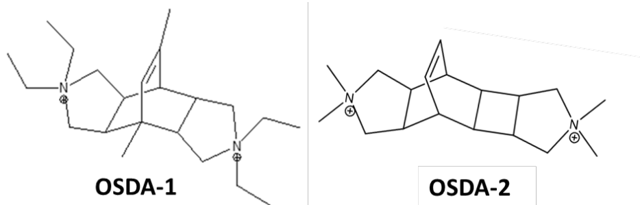
Figure 2: Organic structure directing agents selected to attempt the synthesis of small pore zeolites containing large cavities
