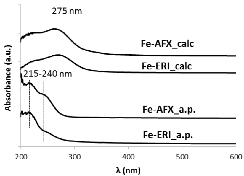
Figure 12: UV-Vis spectra of the as-prepared and calcined one-pot synthesized Fe-containing ERI and AFX samples
