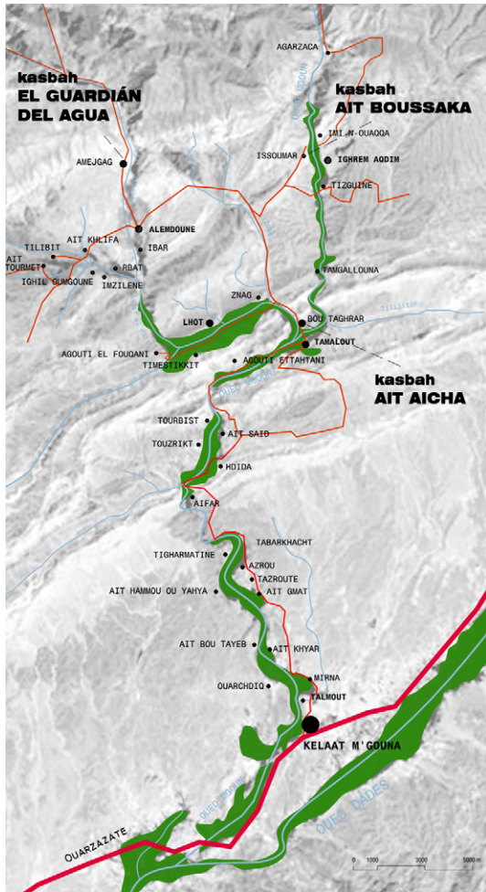
Fig. 2. Map of the M'Goun Valley with the location of the three kasbahs under study.
