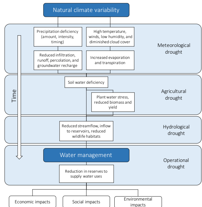
Figure 1. Development chain of droughts through time. Meteorological drought, defined as a lack of precipitation over a region for a certain period of time, develops in the short term. Agricultural drought accounts for the plants and crops water stress; it develops in the medium term. Hydrological drought, defined as a period of low streamflow in watercourses as well as lake and groundwater levels below normal, develops in the long term. Operational drought, defined as a period with anomalous supply failures in a developed water exploitation system, develops in the long term. Figure adapted from Spinoni et al. (2016) to include operational drought.
