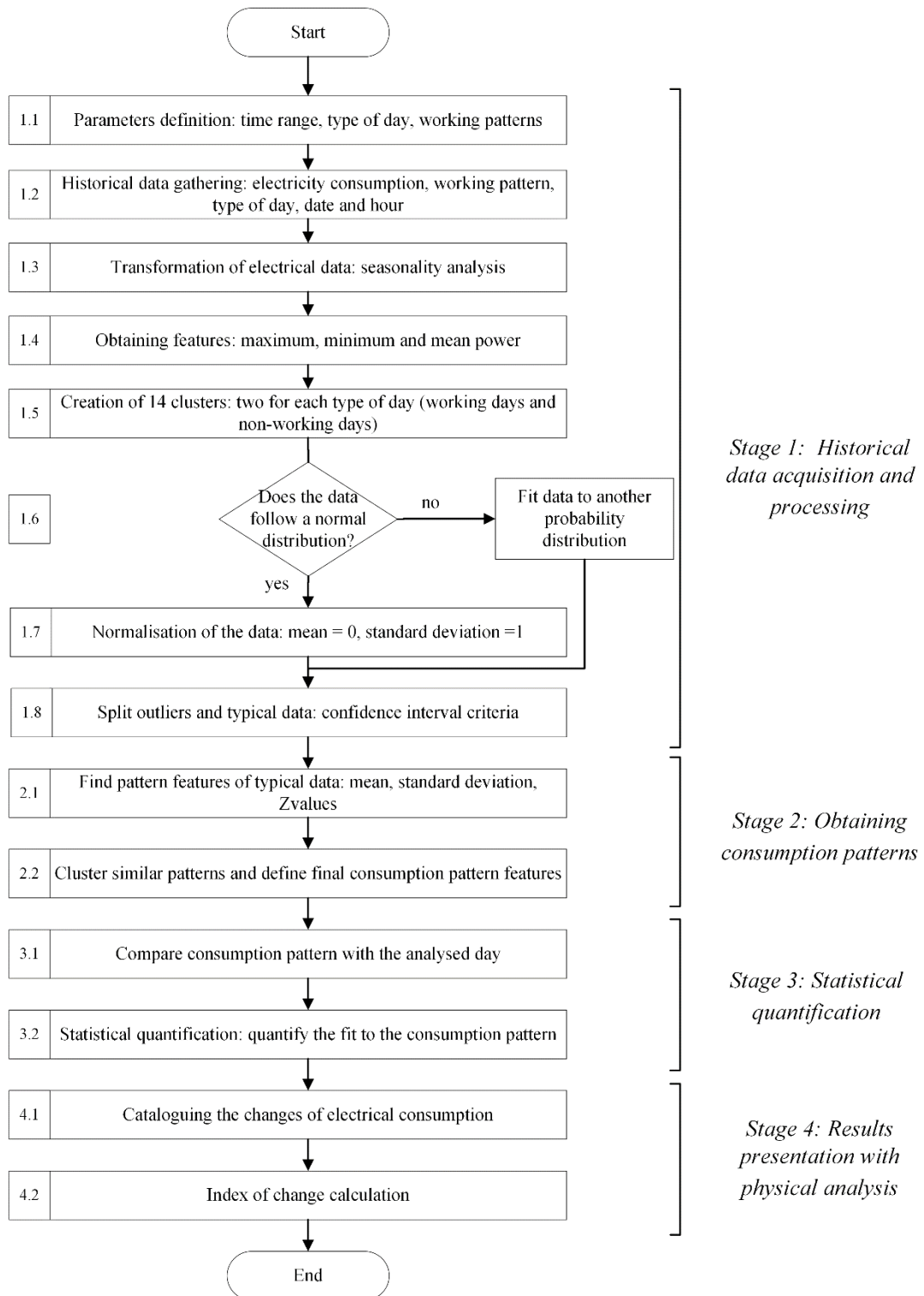
Figure 1. Flowchart of SAICC methodology
