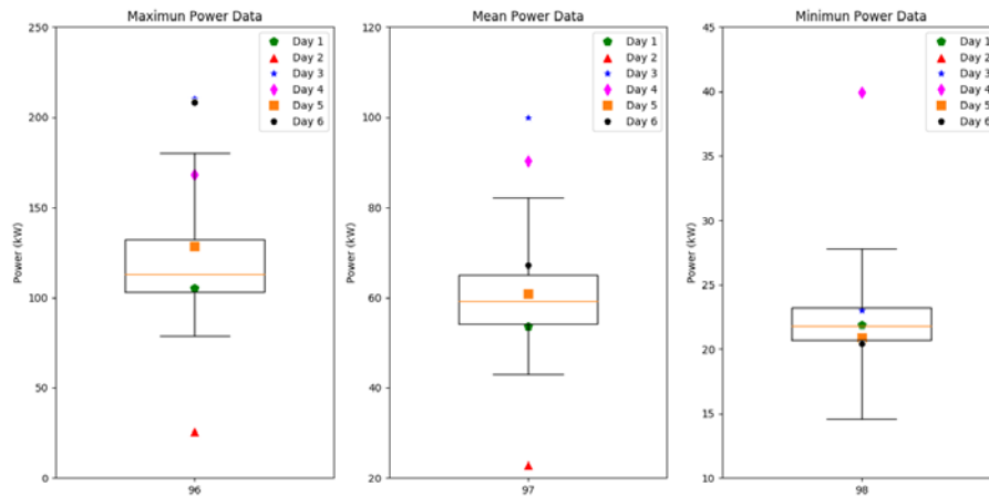
Figure 6. Boxplot of maximum, mean, and minimum power of analysed days
