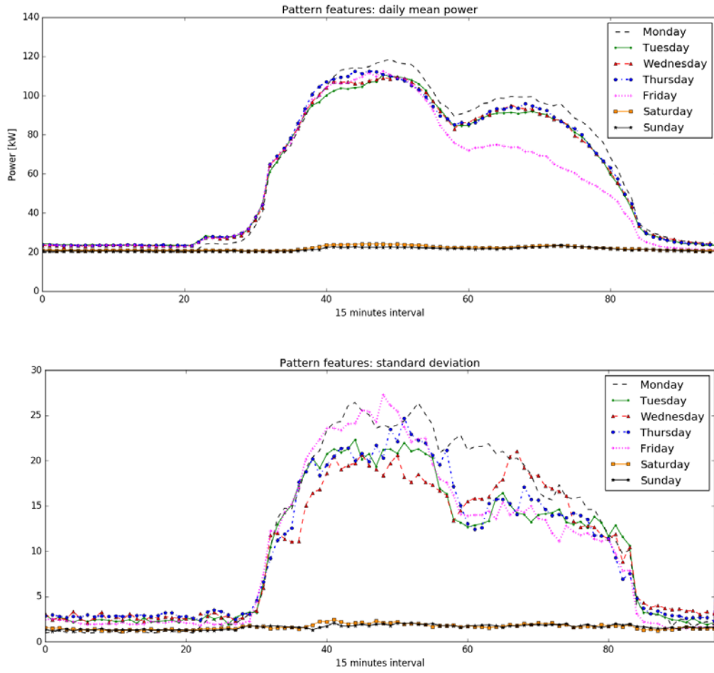
Figure 3. Finding pattern features, mean power, and standard deviation (96 values)
