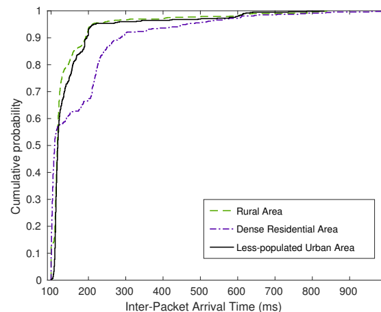
Fig. 13: Cumulative Distribution Function of Inter-Packet Arrival Time.
