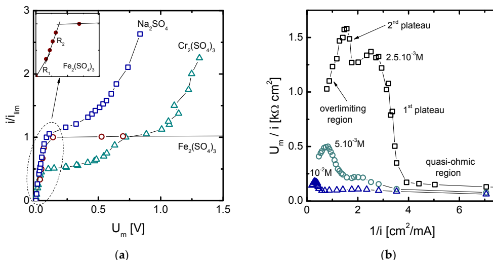
Figure 5. (a) Normalized current-voltage curves obtained for different solutions and (b) Cowan-Brown plot obtained for \text{Cr}_2(\text{SO}_4)_3 solutions of different concentrations.
