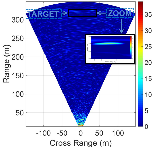
Fig. 32. Range-Azimuth section view of the 3D radar image capture, with 1 corner reflector visible at 315 m.
