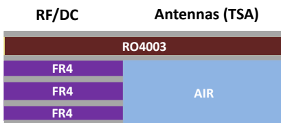
Fig. 4. Representation of the used layer stack-up.
