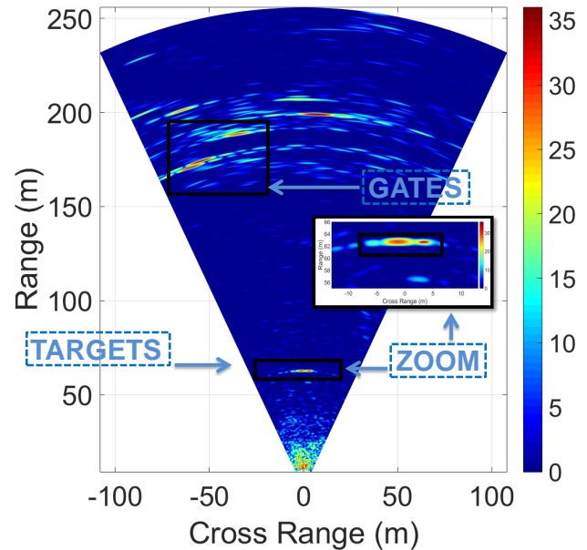
Fig. 21. Range-Azimuth section view of the 3D MIMO radar image capture from the radar setup scenario with two reflectors at a distance of 60\ \text{m} .
