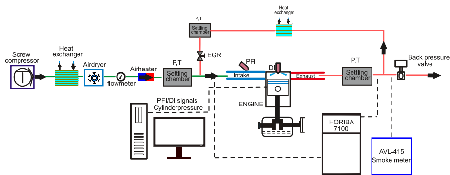
Figure 2. Test cell scheme [43]. EGR: exhaust gas recirculation.
